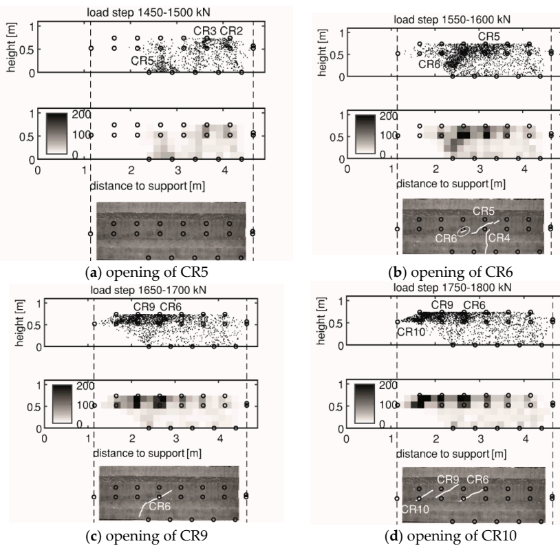
Figure 13. Opening of shear cracks in HPZ04: (a) CR5; (b) CR6; (c) CR9; and (d) CR10. At each subfigure, from top to bottom: the first plot is the estimated location of AE events, the second plot shows the local cumulative AE events, and the third plot shows the incremental crack opening from DIC. The DIC results are edited to help the reader identify the important cracks.
