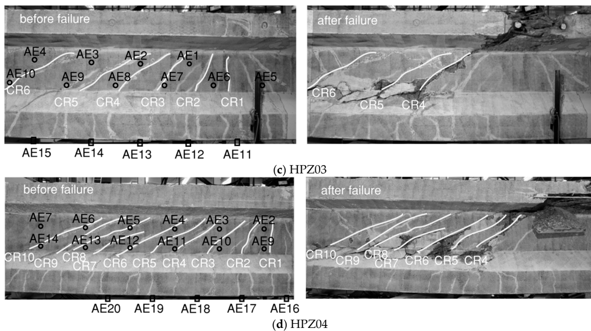
Figure 11. Crack patterns in the four girders from DIC results before and after failure, with the locations of AE sensors: (a) HPZ01, (b) HPZ02, (c) HPZ03, (d) HPZ04.
