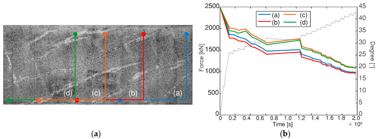
Figure 16. (a) Evaluated areas for HPZ04, and (b) Rotation of the principal strain direction during loading for HPZ04.
