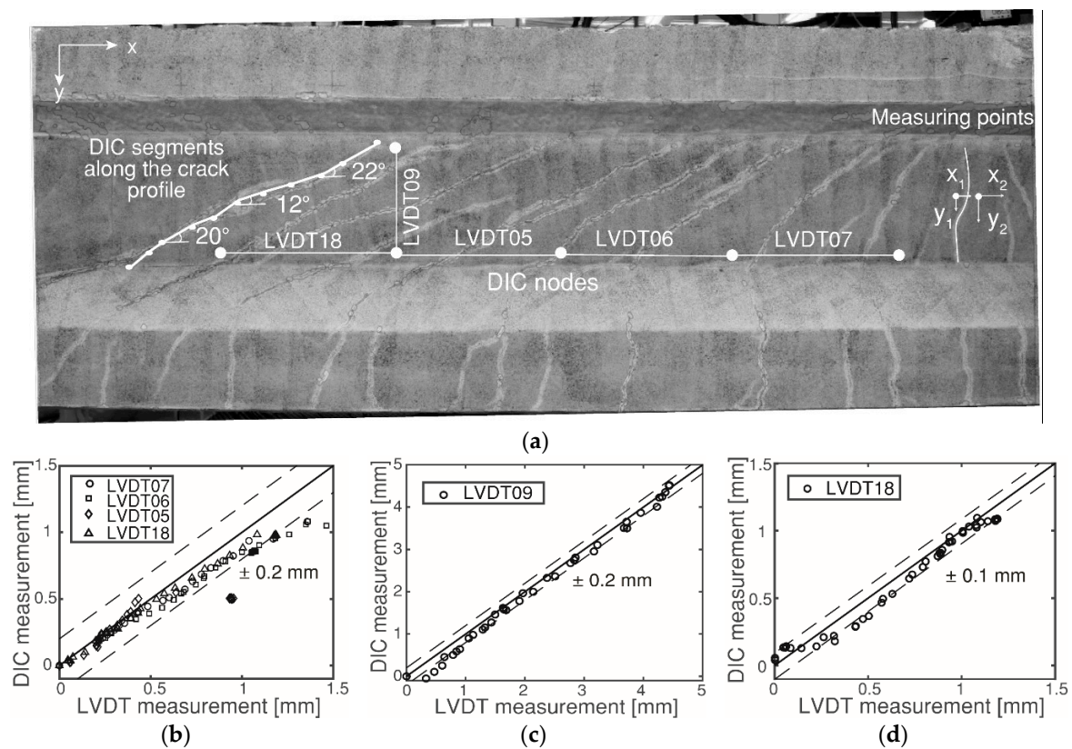
Figure 8. Calibration of DIC with LVDT in HPZ04: (a) location of DIC nodes and LVDTs 05–07, LVDT09, and LVDT18, together with the segmental division in one crack; (b) LVDTs 05–07 and LVDT18 measurements and DIC with Canon 5DS R (20 mm lens); (c) LVDT09 measurement and DIC with Sony A5000; and (d) LVDT18 measurement and DIC with Canon 5D (90 mm lens).
