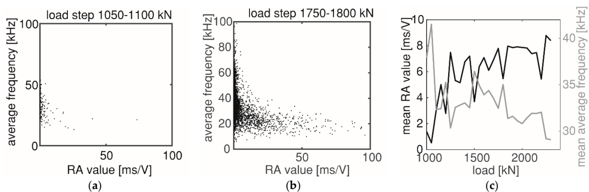
Figure 14. (a,b): Average frequency and RA value of each AE event at load steps 1050–1100 kN and 1750–1800 kN, respectively, and (c): Changing of mean average frequency and mean RA value with loading.
