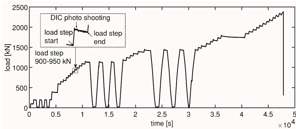
Figure 2. Loading history of HPZ04.
