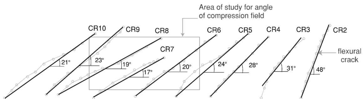
Figure 17. Crack pattern and crack angle from DIC results of HPZ04.
