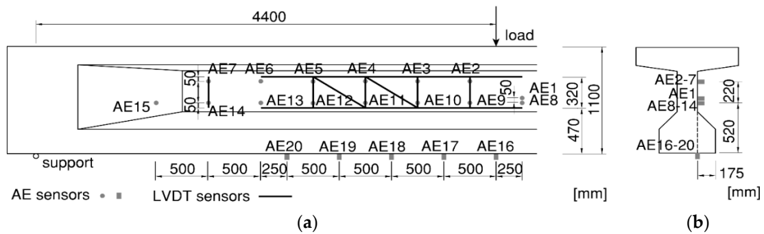
Figure 3. Sensor plan for beam HPZ04 showing LVDTs and AE sensors: (a) Side view; (b) cross-section.
