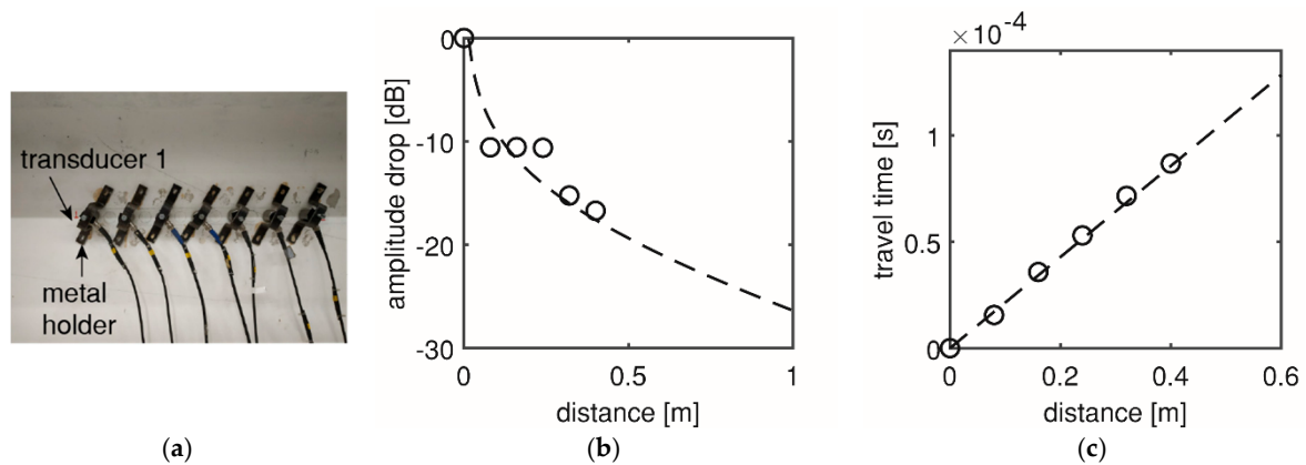
Figure 4. Baseline measurement in HPZ03: (a) Setup, (b) amplitude drop, and (c) wave speed.
