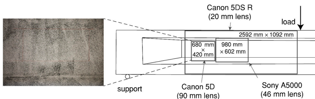
Figure 7. DIC setup for beam HZP04 showing the random pattern, and the position of the 20 mm wide angle lens, the 90 mm lens and the SONY A5000 camera.
