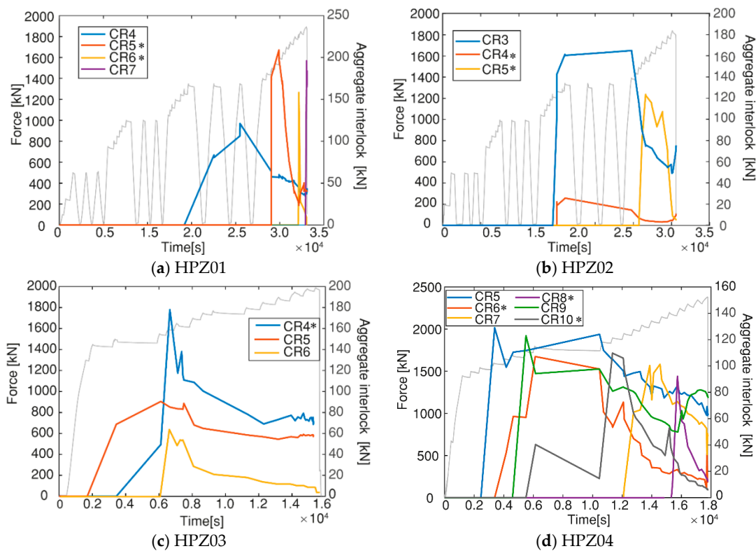
Figure 15. Aggregate interlock contribution during loading analyzed over time for all the experiments: (a) HPZ01; (b) HPZ02; (c) HPZ03; and (d) HPZ04. * indicates the critical shear cracks.
