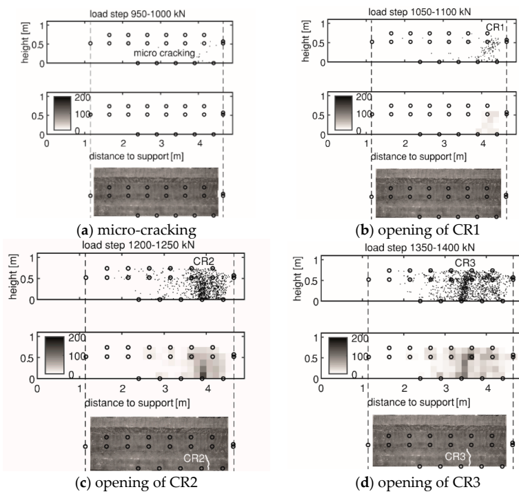
Figure 12. Opening of flexural cracks in HPZ04: (a) Microcracking; (b) CR1; (c) CR2; and (d) CR3. At each subfigure, from top to bottom: the first plot is the estimated location of AE events, the second plot shows the local cumulative AE events, and the third plot shows the incremental crack opening from DIC. The DIC results are edited to help the reader identify the important cracks.
