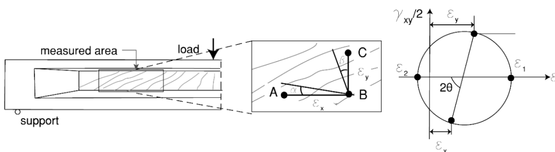
Figure 9. Scheme of measured area for HPZ04 and Mohr's circle for average strains.
