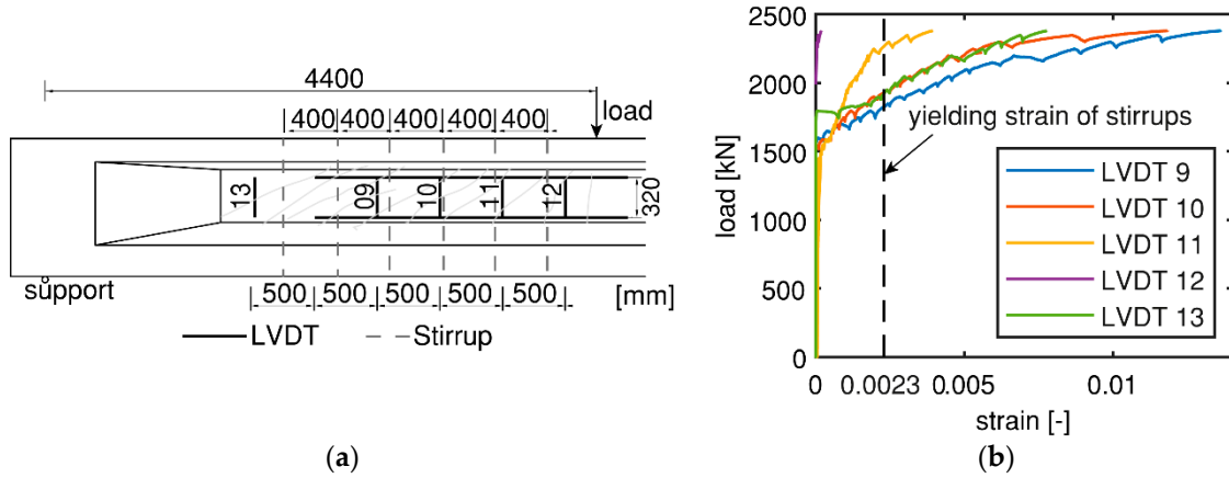
Figure 10. Measurement of yielding stirrups from LVDTs for HPZ04: (a) Position of the stirrups and LVDTs; and (b) Vertical deformation results of LVDTs.
