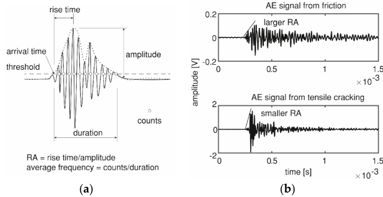
Figure 5. (a) Illustration of AE parameters and (b) AE signals from friction and tensile cracking. Based on the recorded signal arrival times, grid search method was used to estimate the source location [33]. The grid point, of which the calculated arrival times at the sensors were best matched with the recorded arrival times, was determined as the source location [7]. In this paper, the measuring area was discretized into a grid with size 5 \times 5 mm. The mathematical formulation used in source localization can be found in our previous paper [6].
