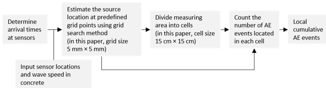
Figure 6. Approach of calculating local cumulative AE events.
