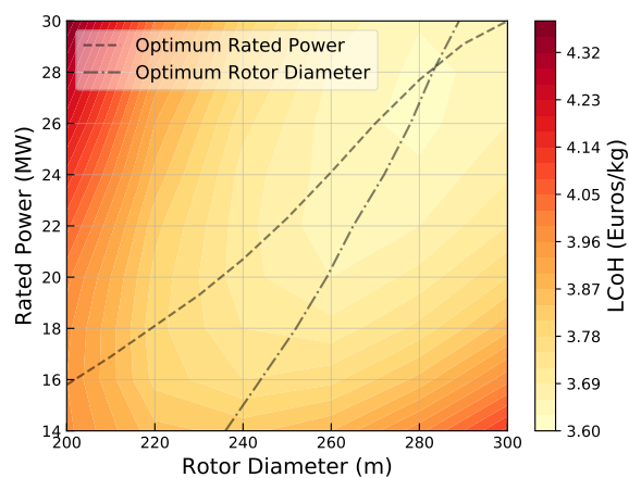
Figure 10: Upscaling results for LCoH: ‘Fixed N_t ’
