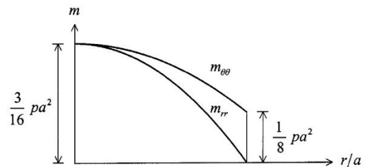
moments of circular slab with load p
