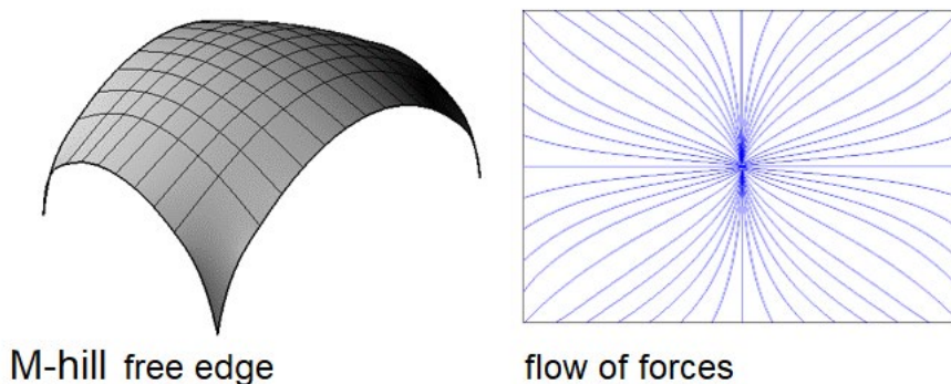
Figure 50 M-hill and its load distribution [images 100]
