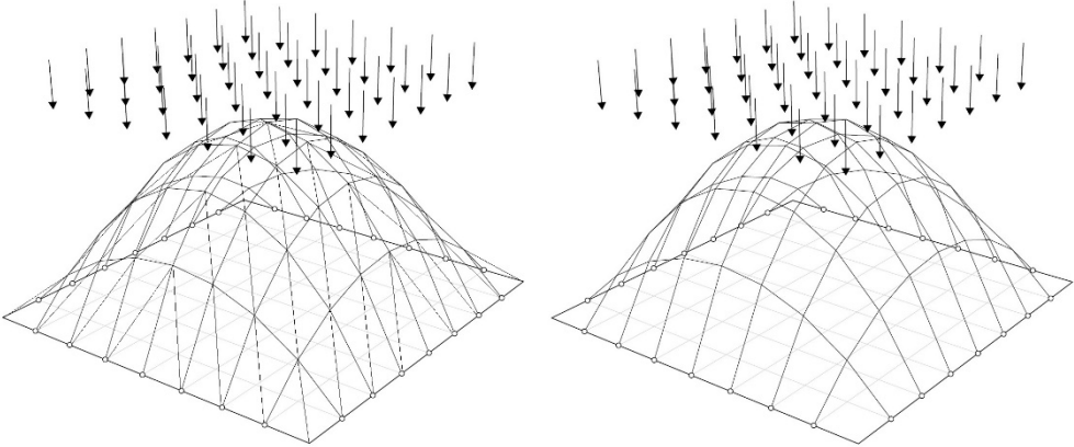
Figure 31 thrust network: left in-plane form stable, right not form stable
