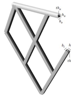
Figure 2 Diagram Façade Components
