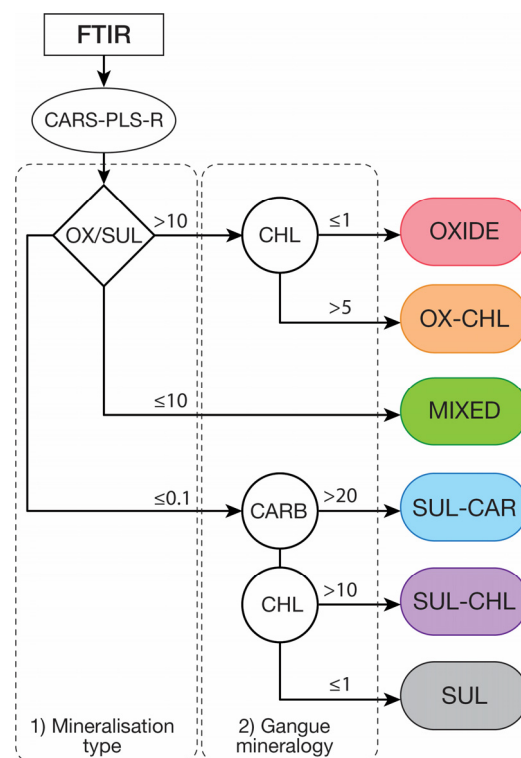
Figure 8. Mineral-based geometallurgical ore type classification scheme proposal using modal mineralogy data obtained from CARS-PLS-R applied to FTIR. OX/SUL: ratio between the amount (in wt.%) of Cu-Co oxide and Cu-Co sulphide minerals, CARB: total amount (in wt.%) of carbonates (Dolomite, ankerite, magnesite) and CHL: amount (in wt.%) of chlorites. Classification thresholds are only indicative.
