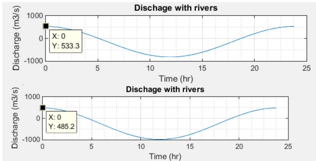
Figure 4-11 The discharge in the fjord - including discharges from the rivers with 95% upper limit. Therefore, the tidal discharge is equal 533.3 \text{ m}^3/\text{s} and 485.2 \text{ m}^3/\text{s} for 10-year and 100-year return periods, respectively
