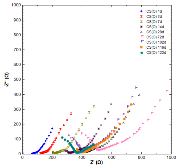
Figure 6. EIS response for CS(O) as an overlay of 1 to 123 days.
