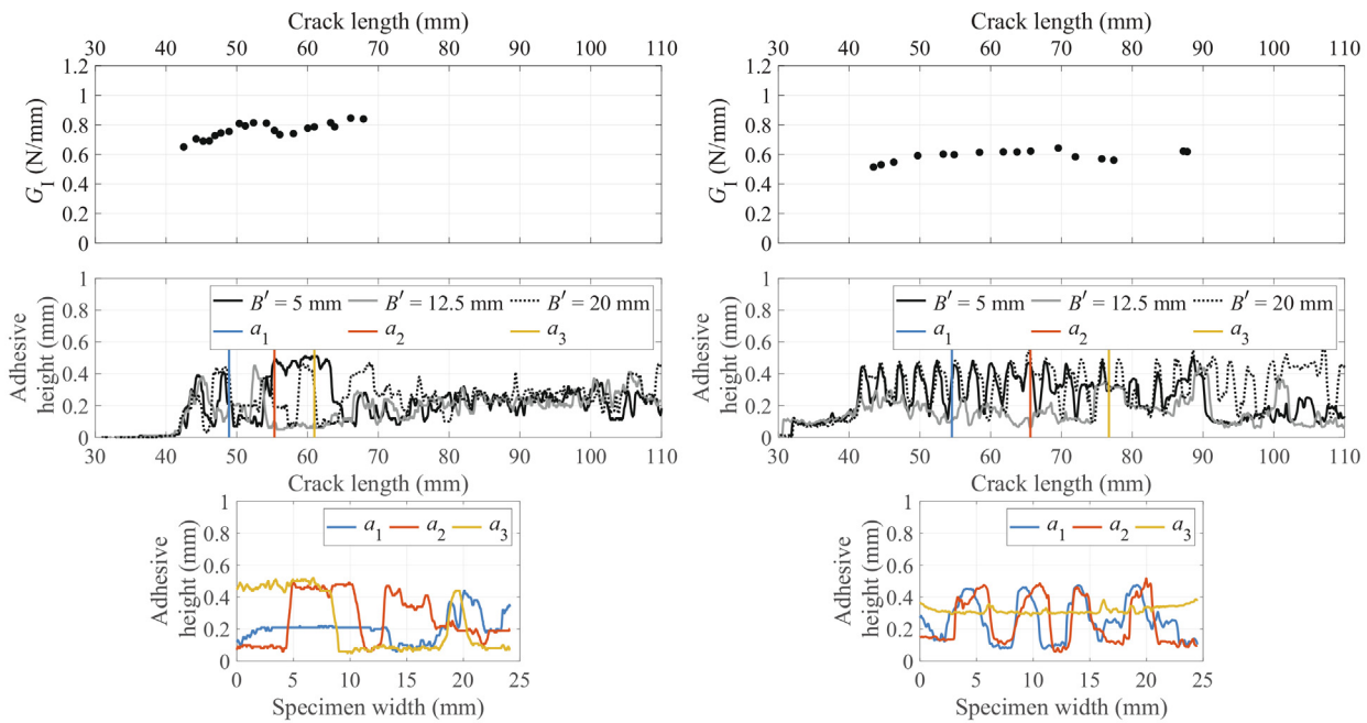
(a) Single-material steel-steel bonded joint. The adhesive height profiles are taken from Arm 1 shown in Fig. 5(a). (b) Bi-material steel-GFRP bonded joint. The adhesive height profiles are taken from Arm 1 shown in Fig. 5(c).
