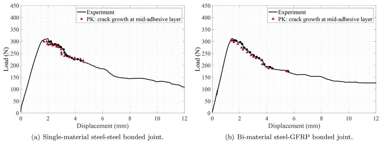
Fig. 9. Representative bonded joints with thin adhesive layer: load-displacement curves.
