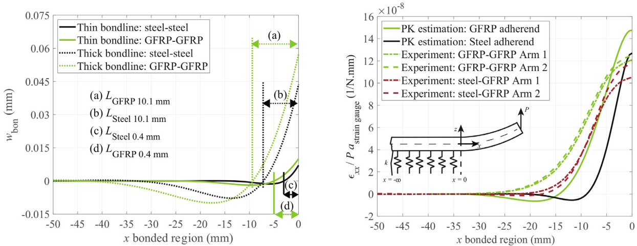
(a) Displacement of PK model in the bonded region, Eq. 4. (b) Experimental results and analytical solutions for normalised longitudinal strain, \epsilon_{xx} , of instrumented DCB joints.
