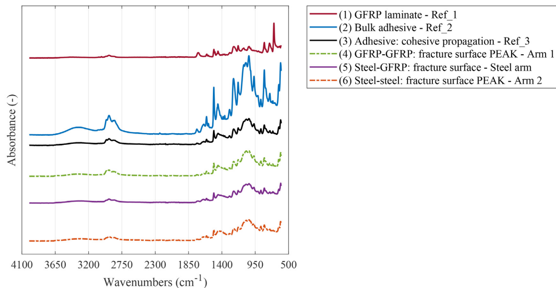
Fig. 7. ATR-FTIR spectra: qualitative comparison.
