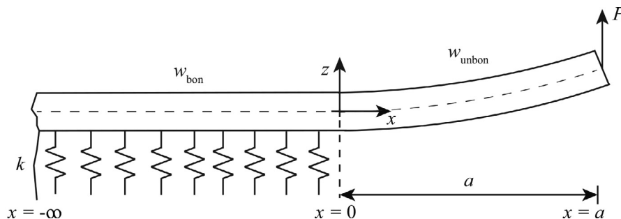
Fig. 4. DCB specimen modelled according to Penado-Kanninen model [39].
