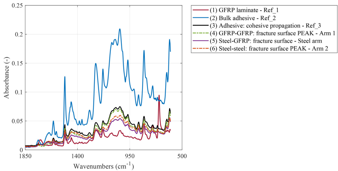
(b) Close-up of the wavenumbers in the range of 1850-500 \text{cm}^{-1} .
