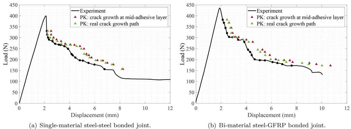
Fig. 10. Representative bonded joints with thick adhesive layer: load–displacement curves.
