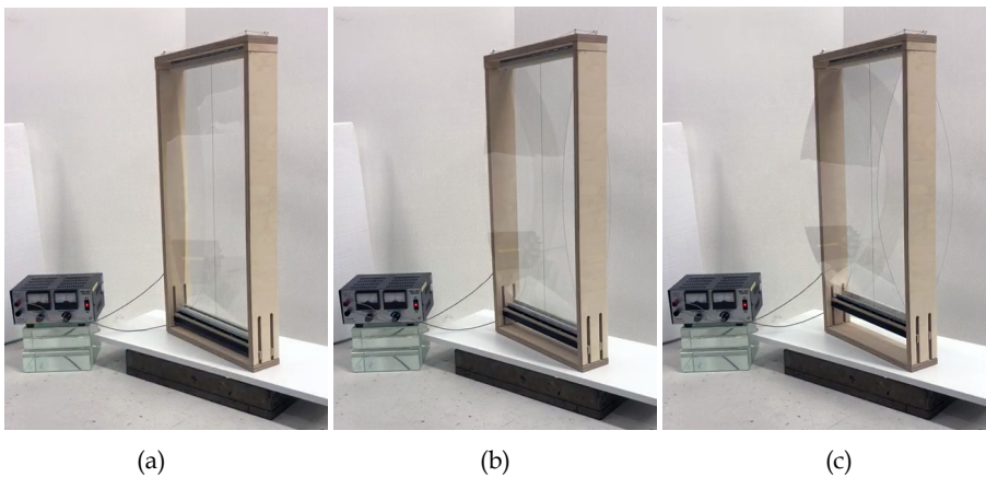
Figure 9: Mock-up of the adaptive thin glass façade concept with shape memory alloy [Miri, 2018]
