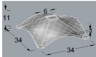
Figure 17: Overview of the thin glass composite panel with 3D printed trussed core [Akilo, 2018]
