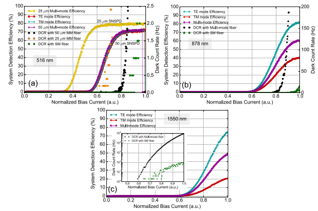
Fig. 3. (a) SDE of 25/50 \mu m diameter SNSPD at 516 nm, (b) SDE of a 20 \mu m diameter SNSPD at 878 nm, and (c) SDE of a 20 \mu m diameter SNSPD at 1550 nm.
