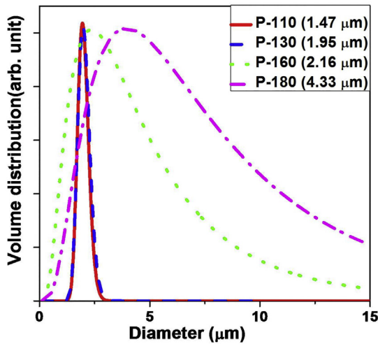
Fig. 2. Granular diameter distribution as obtained from DLS [33].
