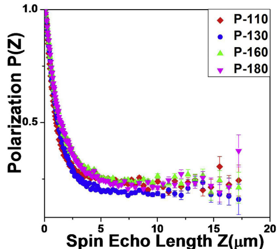
Fig. 3. Depolarization plots obtained from SESANS measurements.
