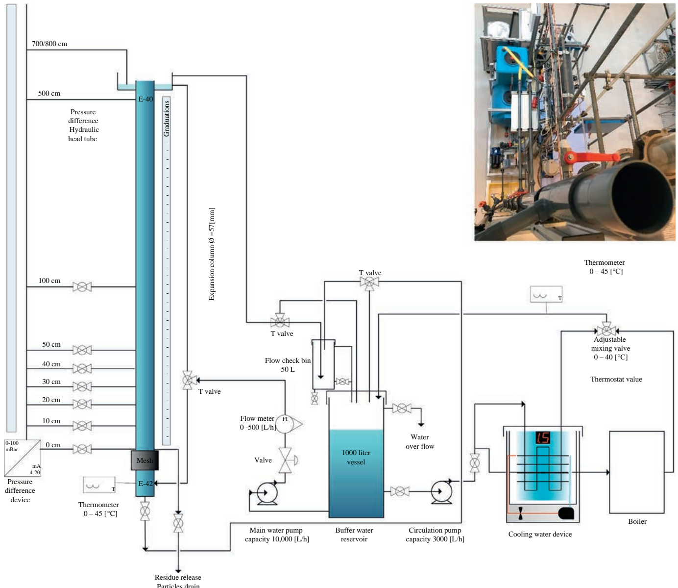
Fig. 5. Experimental setup.
