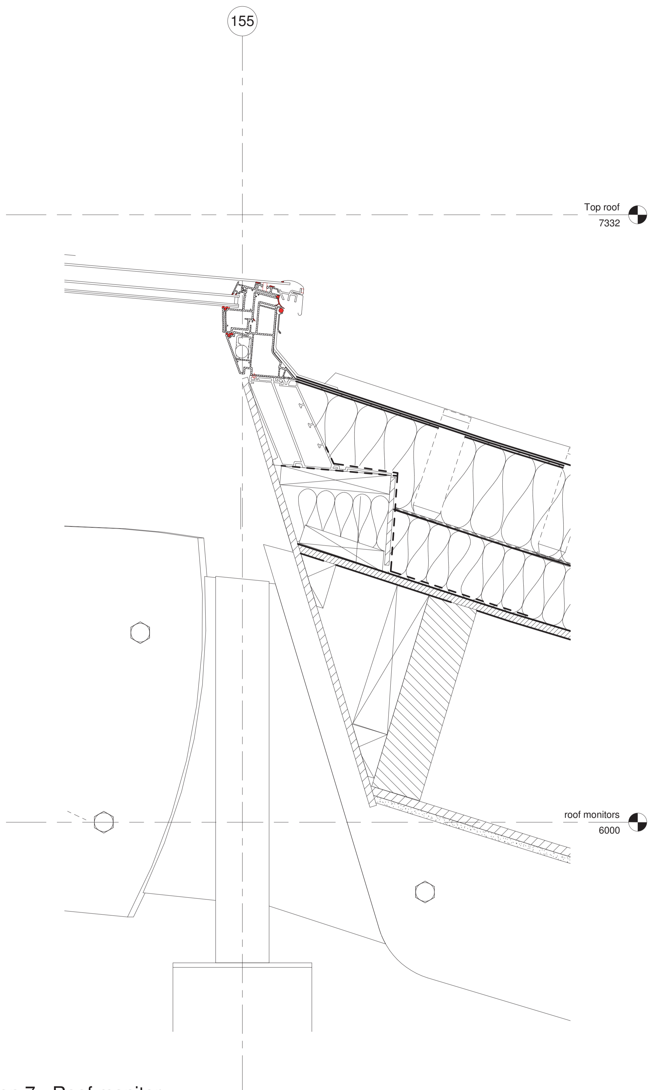
1 - detail 1:5 Section 7 - Roof monitor
