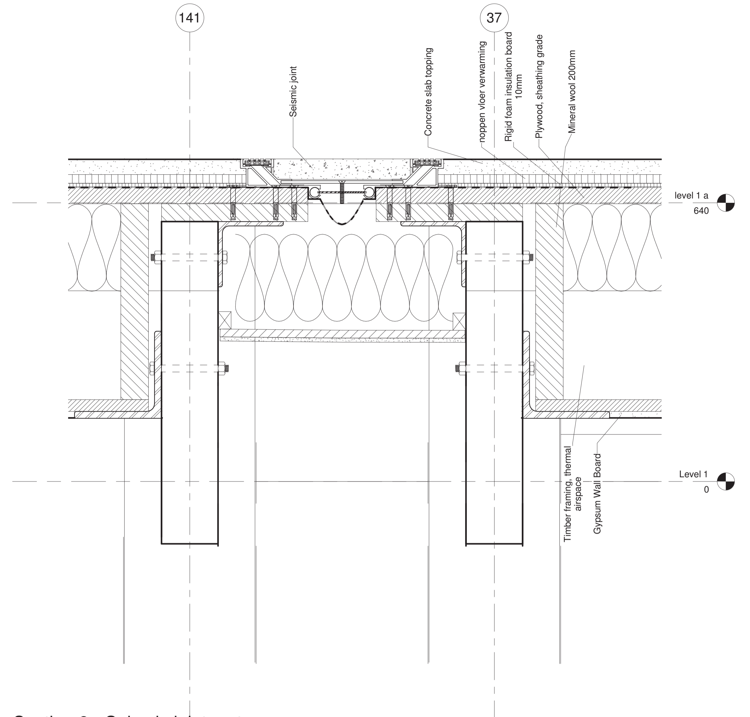
2 - detail 1:5 Section 8 - Seismic joint vert
