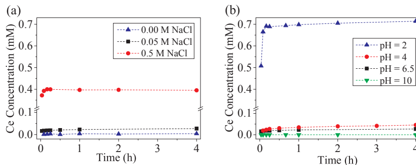
Fig. 6. Ce^{3+} release profiles at neutral pH in different NaCl concentrations (a) and in 0.05 M NaCl at different pH values (b).
