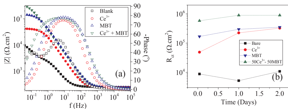
Fig. 1. The EIS spectra after 60 min immersion (a) and evolution of the R_{ct} for AA2024-T3 panels exposed to inhibitor free (■), 1 mM \text{Ce}^{3+} (●), 1 mM MBT (▼) and 0.5 mM \text{Ce}^{3+} + 0.5 mM MBT (▲) containing 0.05 M NaCl (b).
