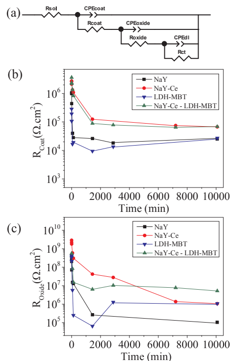
Fig. 9. Equivalent circuit used to fit the experimental EIS data (a), and coating ( R_{coat} ) (b) and oxide ( R_{oxide} ) resistances (c) result of the fitting process of the waterborne coatings immersed for 7 days.
