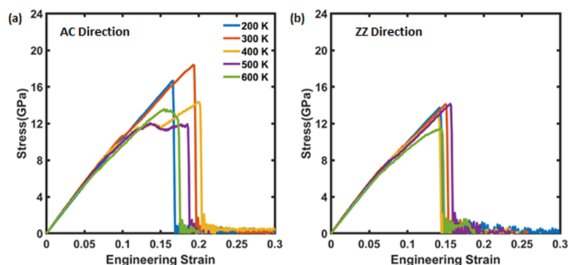
Figure 11. Stress–strain curve of uniaxial tension simulation in the defect-free monolayer WS_2 at various temperatures: (a) loading along the AC direction; (b) loading along the ZZ direction.
