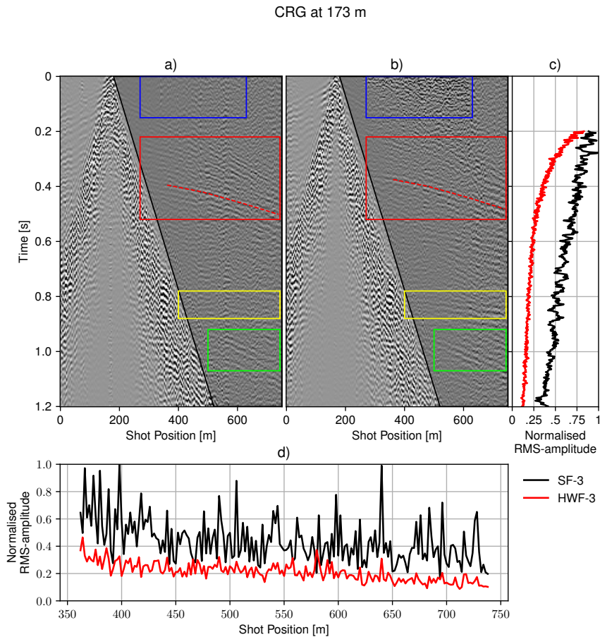
Figure 4.13: CRG at 173 m of a) SF-3 and b) HWF-3 and c) show normalized RMS amplitude as a function of time, calculated outside the surface-wave cone, as highlighted by the dark grey polygon. d) RMS values calculated along the reflection traced by the dashed red line within a 20 ms window. Normalized RMS-amplitude for SF-3 and HWF-3 calculated as: RMS(SF-3)/\max(RMS(|SF-3|)) and RMS(HWF-3)/\max(RMS(|SF-3|)) , respectively.
