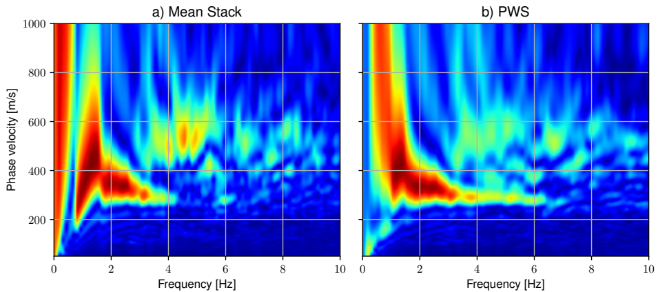
Figure 5.15: Resultant dispersion images of the SF data from mean stacking (a) and phase-weight stacking (b).
