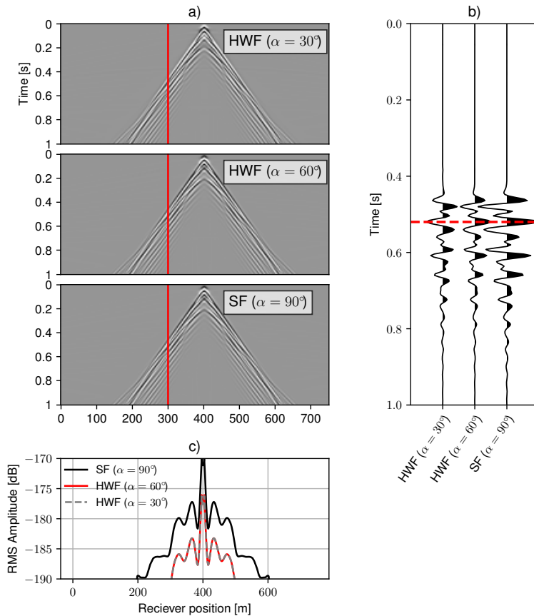
Figure 4.11: a) Modeled surface-wave responses of straight and helically wound fibres with angles and their respective RMS amplitude (c). b) Traces at receiver 300 m (highlighted by the red line in a) showing a comparison between the signals of fibres with different wrapping angles.
