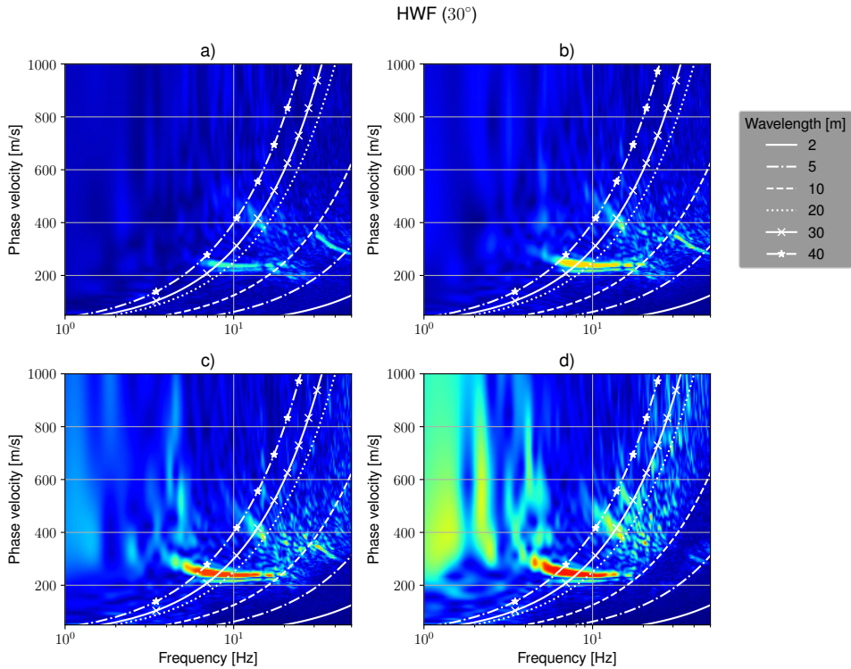
Figure 5.10: HWF ( \alpha = 30^\circ ) dispersion images estimated from the field data with different gauge lengths: a) Dispersion image using data with L_g = 2 m, b) L_g = 5 m, c) L_g = 10 m and d) L_g = 20 m.
