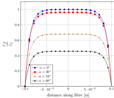
Figure 2.3: Strain transfer factor \xi ( =\varepsilon_f/\varepsilon_c ) for different fibre angles along a fibre length of 0.2 m. Note that this model assumes two fixed ends, which is not the case for our embedded sinusoid. The important thing here is to highlight the effect of the angle.
