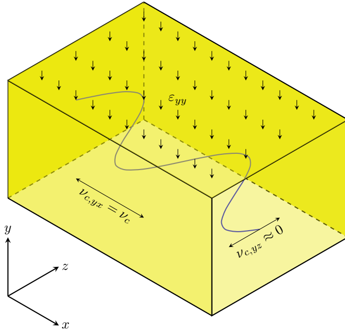
Figure 3.2: Concept of sinusoidally shaped fibre embedded in cable with low-Poisson's ratio \nu_{c,yz} in z -direction due to broadside strain ( \epsilon_{yy} ).
