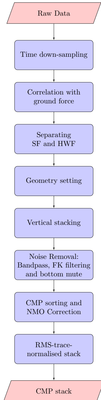
Figure 4.6: Processing flow to produce a CMP stack.
