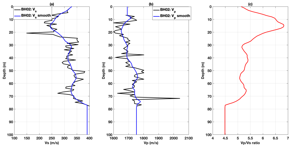
Figure B.9: shear-wave velocity profile (a) and p-wave velocity profile (b) measured at the second borehole (BH02). The blue curves are the smooth version of the original velocity profiles using a moving average filter. (c) The \frac{V_p}{V_s} ratio is computed based on the smooth blue curves.
