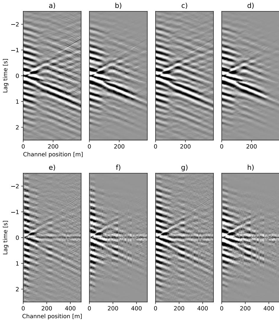
Figure 5.14: Virtual shots with interferometry using different data normalisation and stacking methods. The top row shows SF data with the following: Raw data + Mean stacking (a), Raw data + PWS (b), 1-bit norm. data + Mean stacking (c), 1-bit norm. data + PWS (d). The bottom row contains the HWF data: Raw data + Mean stacking (e), Raw data + PWS (f), 1-bit norm. data + Mean stacking (g), 1-bit norm. data + PWS (h). PWS = Phase-weighted stacking
