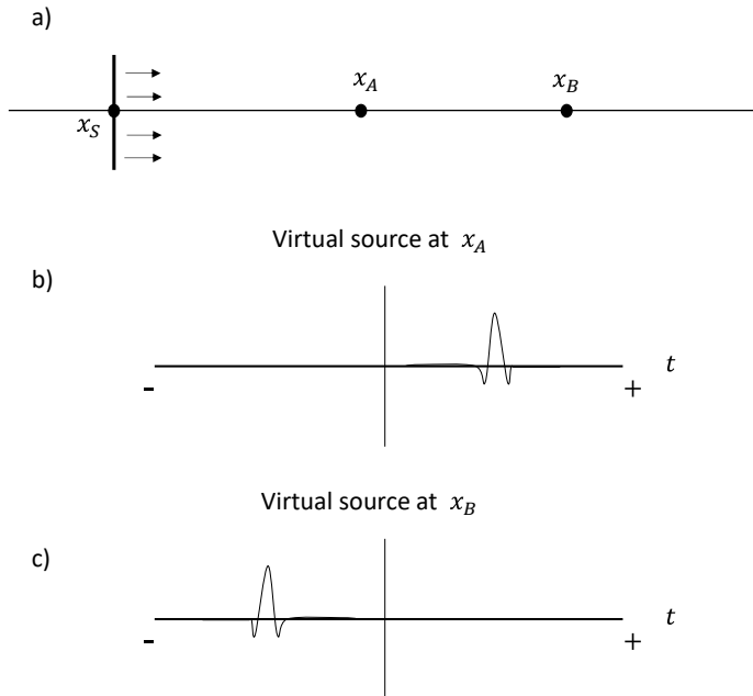
Figure 5.13: Illustration of 1D interferometry: a) shows a plane wave source at x_S , and receivers at x_A and x_B . b) Cross-correlation function at x_B for a virtual source at x_A . c) Cross-correlation function at x_A for a virtual source at x_B .
