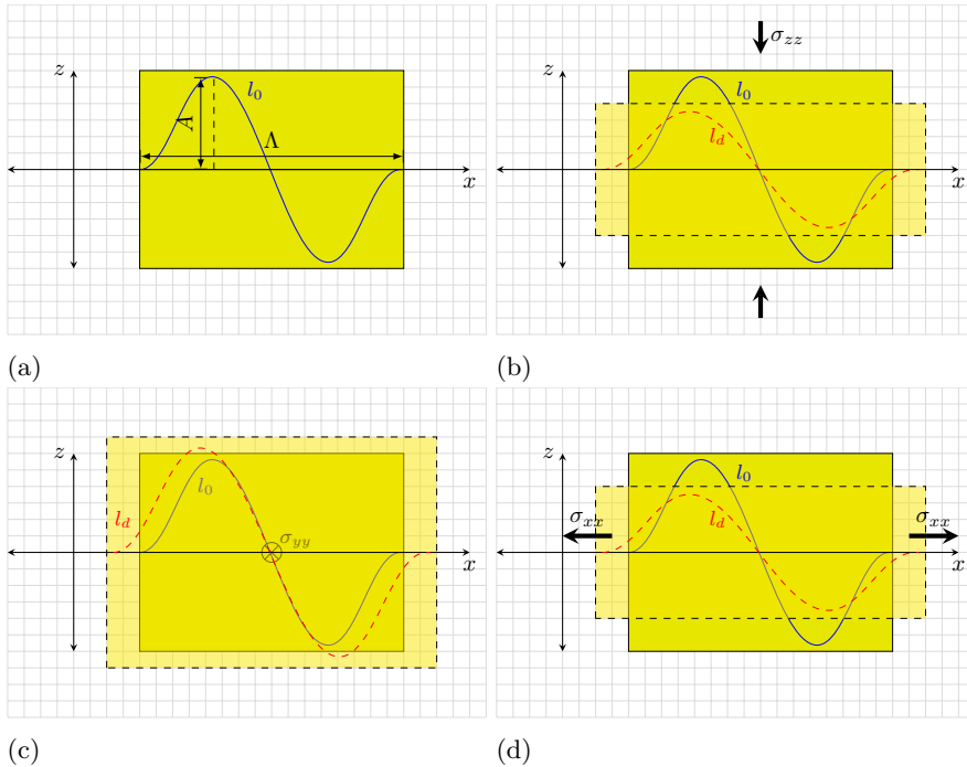
Figure 2.1: Deformation of sinusoid embedded in a strip (a) before deformation, and after (b) in-line deformation and (c) broadside deformation and (d) along-strip deformation.
