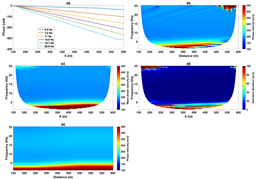
Figure B.3: Phase velocity retrieval using MOPA: application to synthetic recordings. (a) Phase versus offset for six discrete frequencies of the filtered shot record presented in Figure B.2d. (b) Phase velocities c(f_i, x_j^{(c)}) retrieved from one single shot record. (c) Mean local phase velocities retrieved from 32 shots. (d) Standard deviation corresponding to (c). (e) Theoretical (true) laterally varying phase velocities.
