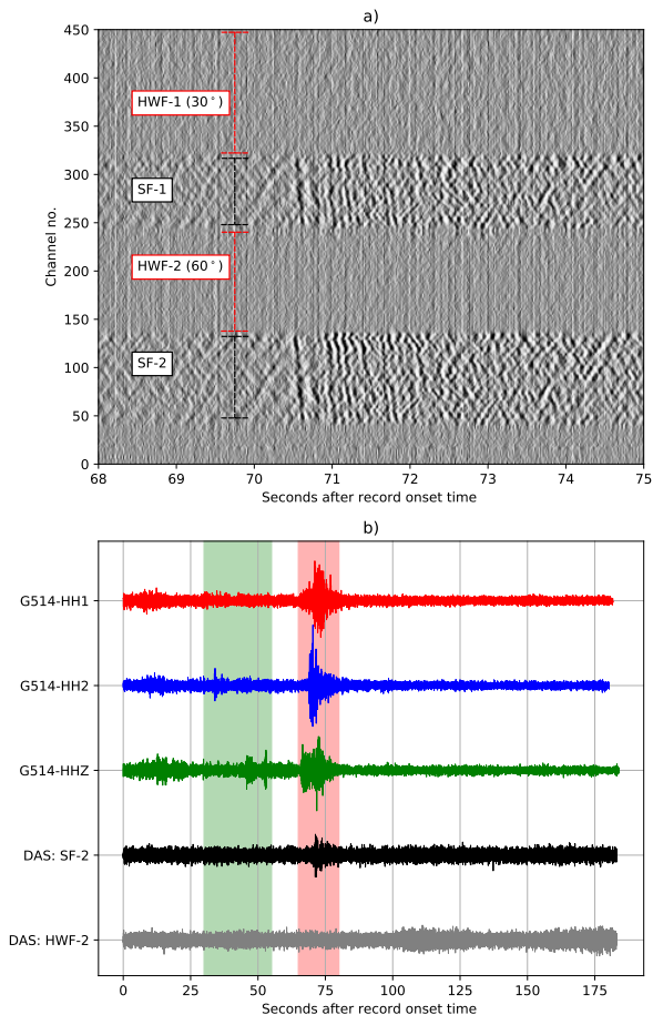
Figure 5.11: Earthquake recording in Zuidbroek, Groningen; date: 18-12-2021, magnitude: 1.3 [KNMI, 2022]: a) DAS Earthquake Recording(record onset time: 02:32:22 UTC) and b) Zuidbroek G514 seismometers vs. DAS (record onset time: 02:32:24 UTC).
