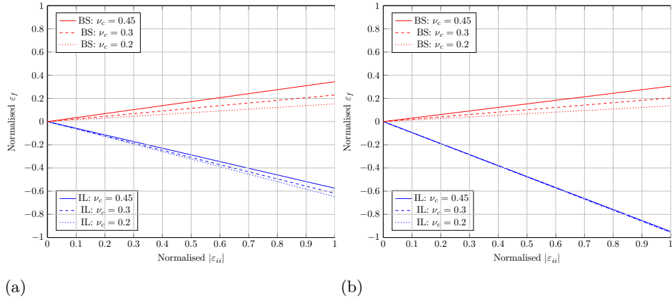
Figure 3.3: Fibre strain \varepsilon_f for broadside (BS) and in-line (IL) orientations, normalised by the maximum applied strain, as a function of in-line normalised applied strain for various Poisson's ratios with (a) A = 2.4 and \Lambda = 6 (in cm) and (b) A = 4.8 and \Lambda = 6 (in cm)
