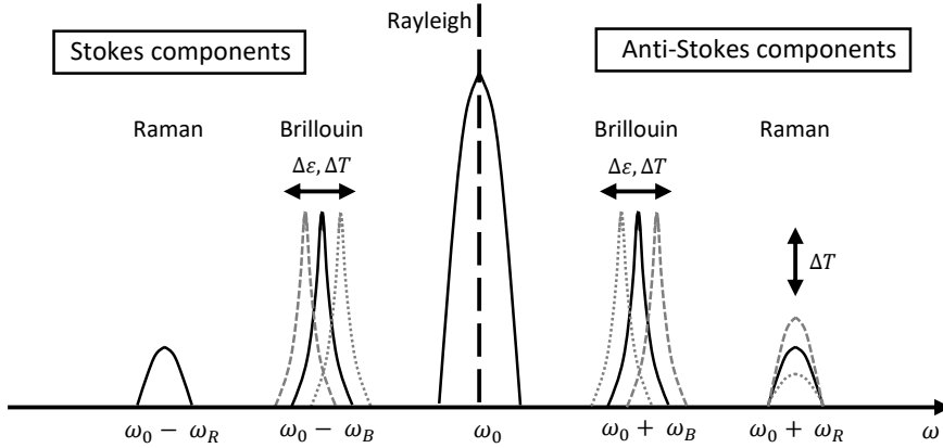
Figure 1.3: Effect of strain \Delta\varepsilon and temperature \Delta T changes on the scattering in optical fibres (modified from Muanenda et al. [2019])
