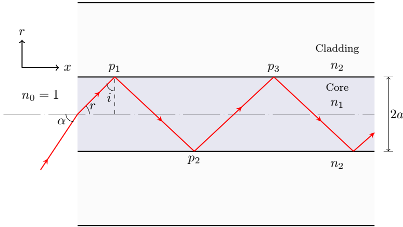
Figure 1.2: Internal reflection of light in step-index optical fibre.
