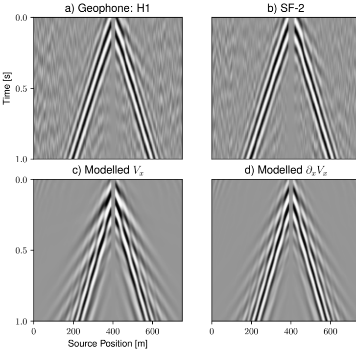
Figure 4.7: Common-receiver gathers at 400 m; recorded geophone H_1 (a), recorded SF-2 (b), modelled V_x (c), modelled \partial_x V_x (d).
