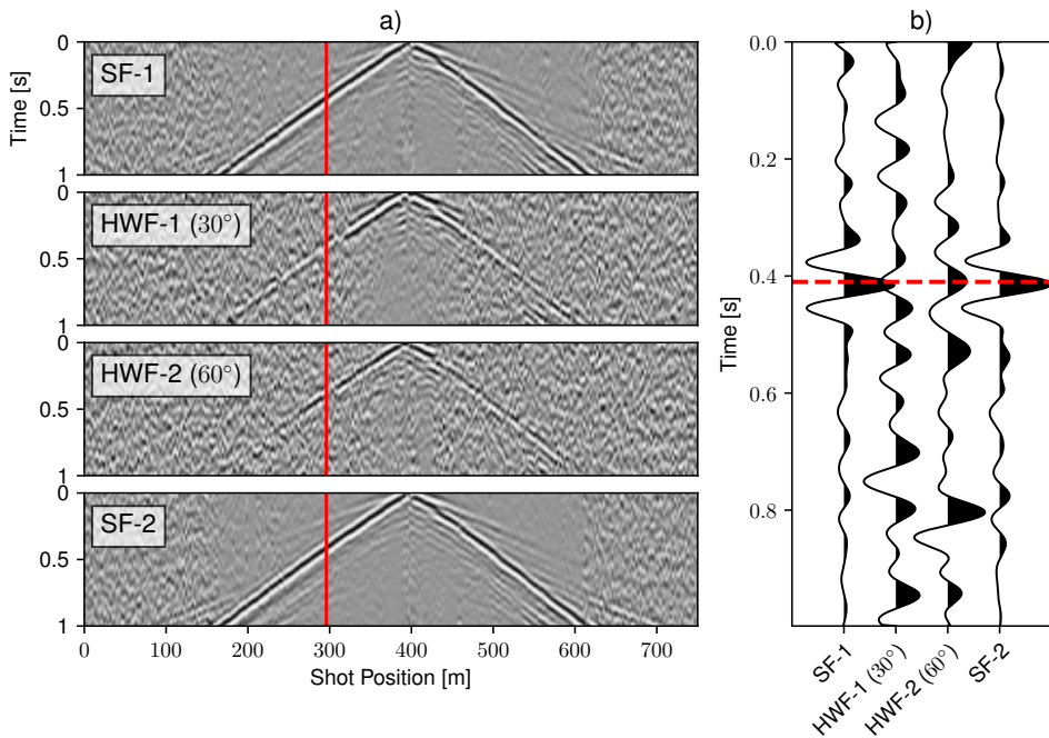
Figure 4.10: a) Recorded common receiver gathers at 400 m of fibres: SF-1, HWF-1, HWF-2 and SF-2. b) Traces at shot position 298 m (marked by the red line in a) showing a comparison of signals from the same offset for the different fibre configurations.
