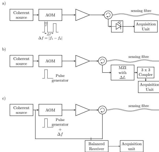
Figure 1.8: System set-up of common DVS/DAS interrogation approaches adapted from Masoudi and Newson [2017a]: a) Dual-pulse, B) Single-pulse and C) Heterodyne. AOM in the figure stands for acoustic-optic modulator.
