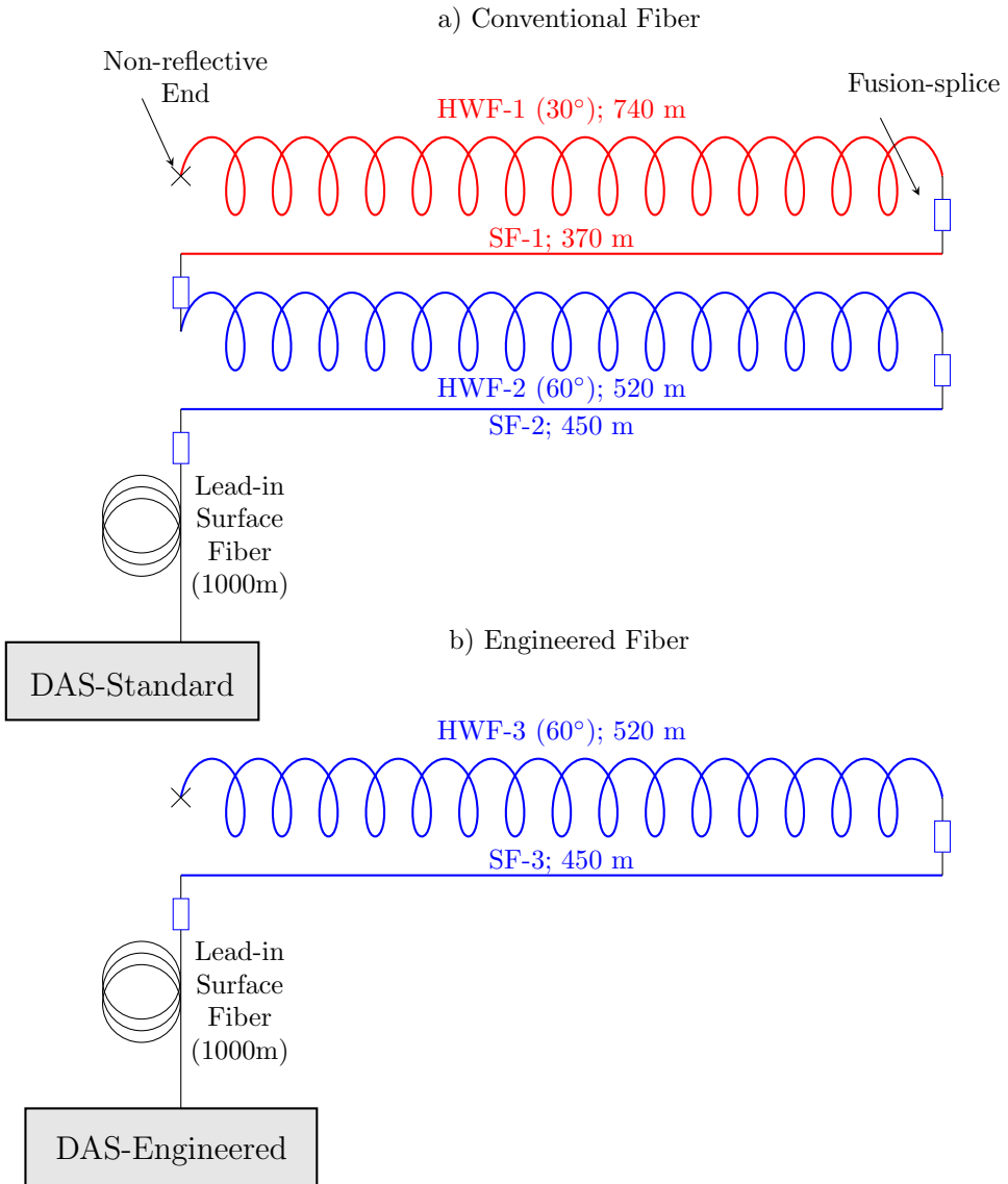
Figure 4.4: DAS systems and fibre configurations; a) DAS-Standard system connected to conventional fibres and b) DAS-Engineered system connected to engineered fibre.
