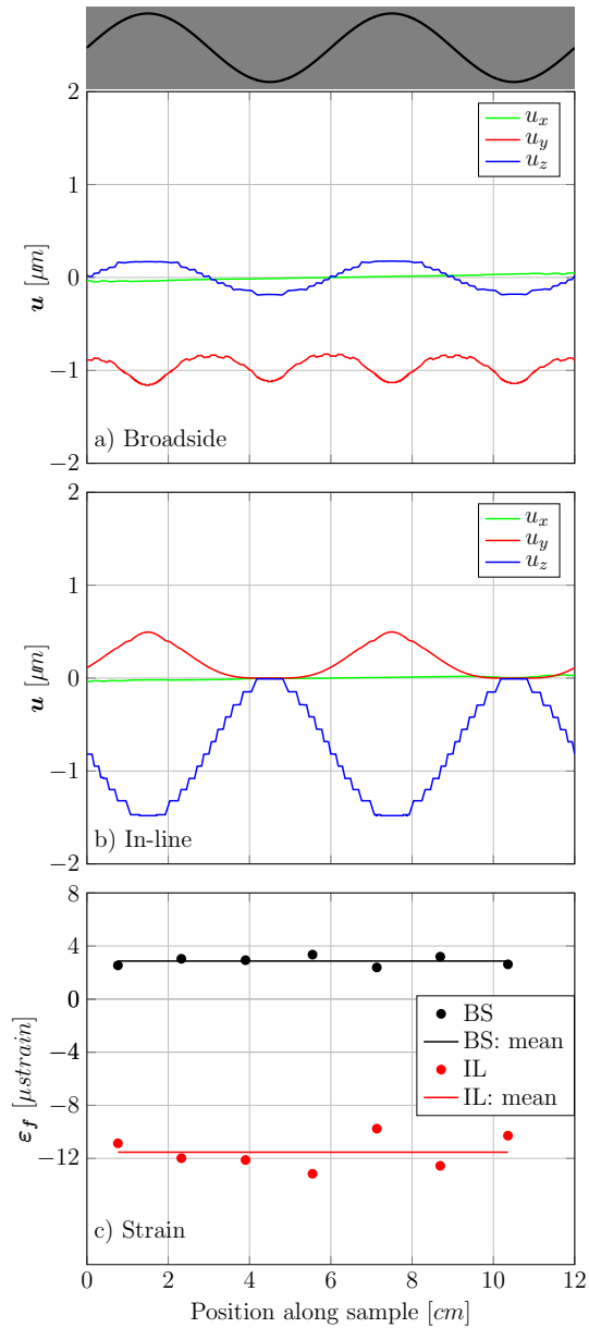
Figure 3.11: Finite element modelling results show the displacements due to broadside (a) and in-line (b) loads and strain measured along the embedded fibre for both loading scenarios (c).
