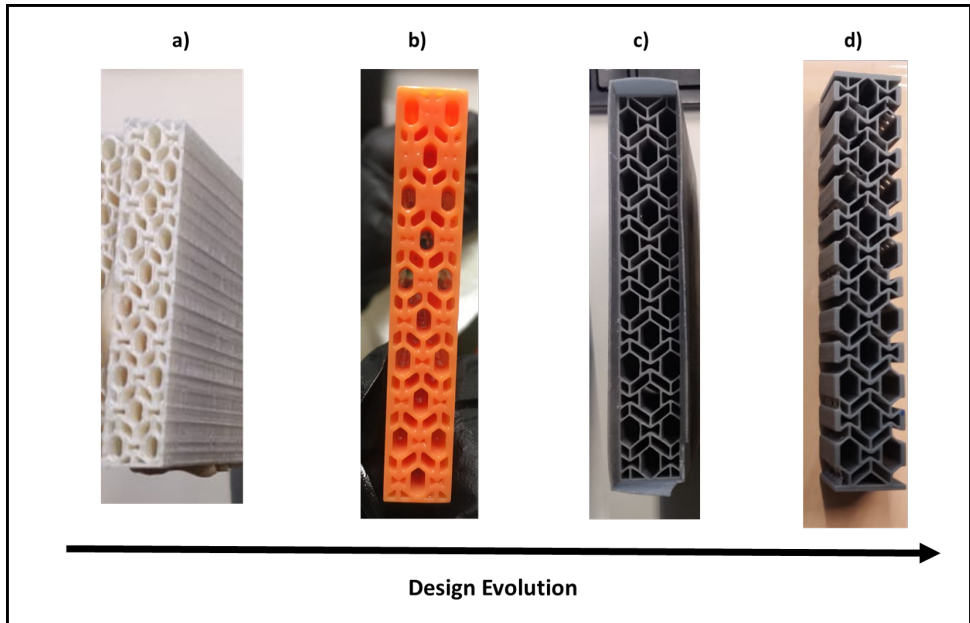
Figure 3.5: Design evolution of 3D-printed low-PR samples. a) Stiff-material print (made of Polylactic acid); b) low-quality resin print; c) high-quality resin print; d) adapted design.
