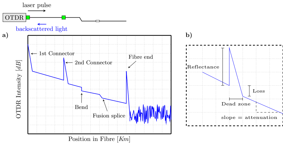
Figure 1.4: Idealised OTDR Example Trace.
