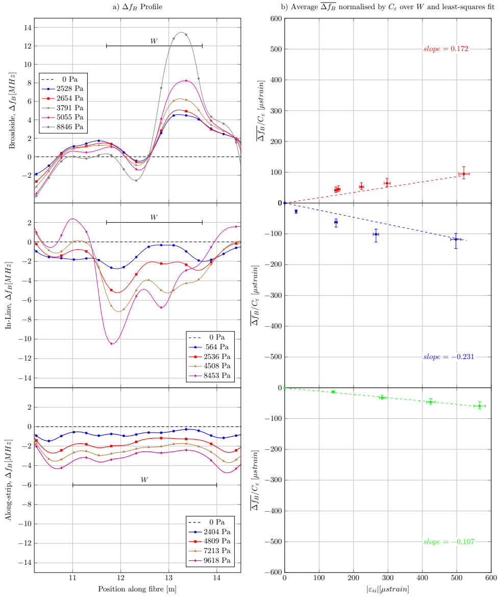
Figure 2.8: Analysis of differences in Brillouin frequency shift. a) Differences in profiles compared to the reference (zero-load) case, with analysis window W indicated. b) \overline{\Delta f_B}/C_\epsilon in \mu\epsilon (dots) as a function of applied strain, where bar above \Delta f_B means average over window W . Dashed lines are least-squares linear fits with slopes, i.e., sensitivities, given; corrections for intercept afterwards applied to force the lines to go through the origin.
