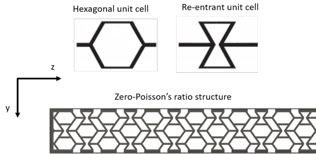
Figure 3.4: low-Poisson's ratio structure using hexagonal and re-entrant ("diabolo"-shaped) unit cells.
