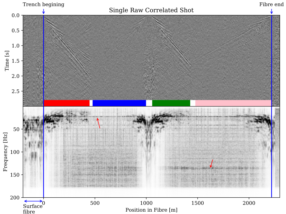
Figure 4.5: Correlated single raw shot of DAS-Standard system in time-distance (top) and frequency-distance domain (bottom). Portions of fibre coloured in red, blue, green and pink correspond to fibres SF-2, HWF-2, SF-1 and HWF-1, respectively; white portions are splices.
