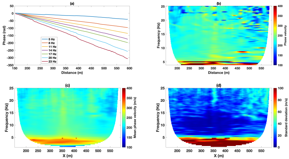
Figure B.7: MOPA applied to the field DAS data considering the lateral variation of the subsurface. (a) Unwrapped phase versus offset at seven different frequencies (i.e., different colors) for the filtered seismic record depicted in Figure B.6d. (b) laterally varying phase velocity retrieved from the single shot record of Figure B.6d. (c) Mean of the laterally varying dispersion curves retrieved from 152 off-end shots. (d) Standard deviation corresponding to (c).
