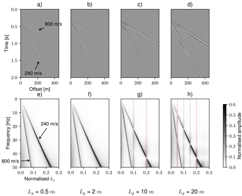
Figure 5.4: Time-distance (top) and frequency-wavenumber (bottom) plots of two events of 240 and 800 m/s, for different gauge lengths. The channel spacing is kept at 0.5 m for all the synthetic shots. The red dotted lines in g and h panels indicate the theoretical positions of the notches at every n/L_g .
