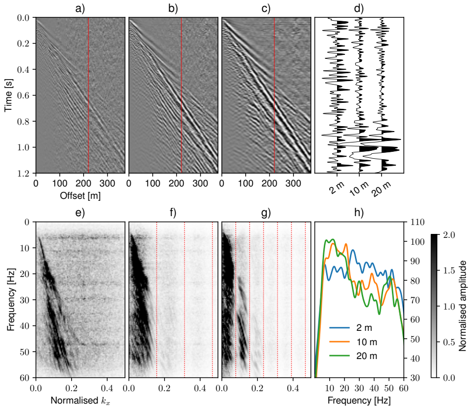
Figure 5.6: HWF ( \alpha = 30^\circ ) field data with gauge lengths 2 m (a), 10 m (b) and 20 m (c), and their respective (f, k_x) spectra, 2 m (e), 10 m (f), 20 m (g). Traces at offset 220 m from different gauge lengths (d) and their amplitude spectra in dB scale (h). The red dotted lines in the f and g panels indicate the theoretical positions of the notches at every n/L_g .
