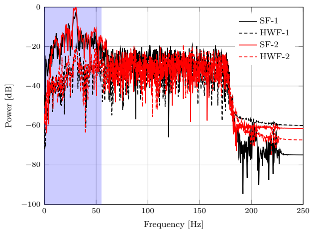
Figure 4.9: Power spectra of portion inside the surface-wave cone of CRG at 400 m (shot positions: 328-336 m) for different fibre configurations. Band 2-55 Hz is highlighted to indicate the main differences between HWF and SF amplitudes.
