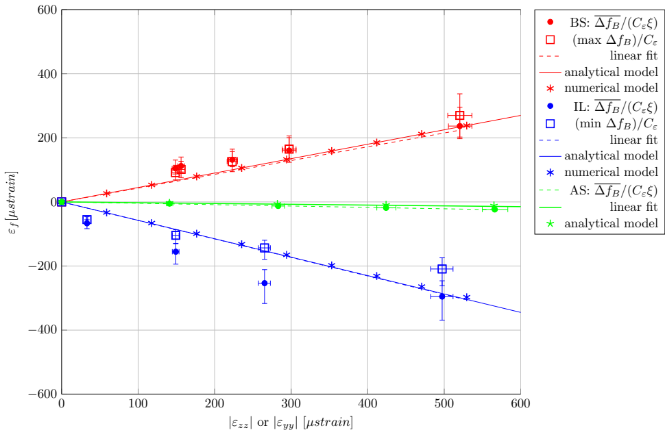
Figure 2.9: Comparison between measured ( = \overline{\Delta f_B}/(C_\varepsilon \xi) ) and modelled \varepsilon_f for in-line and broadside orientations.
