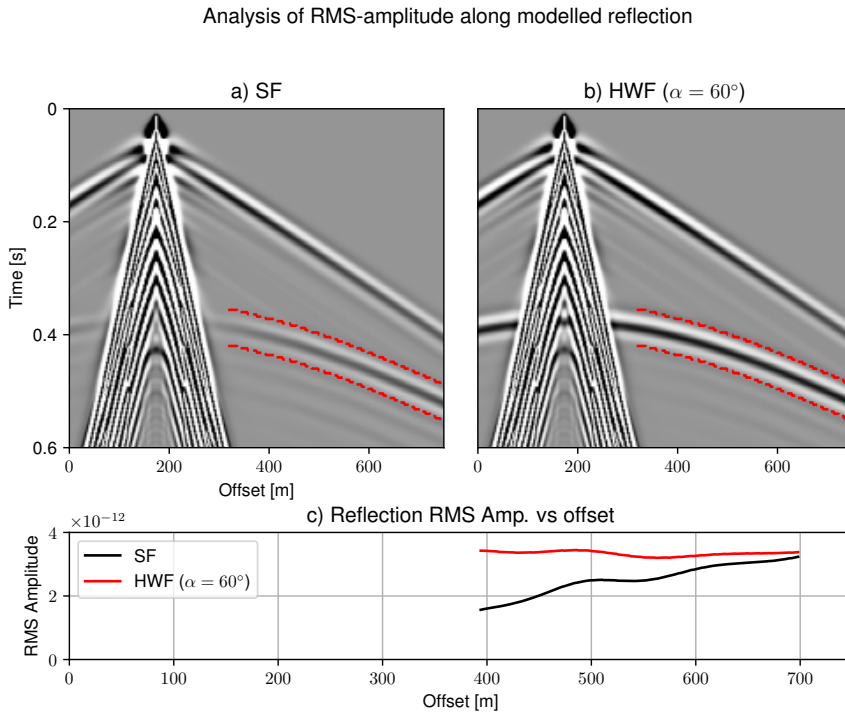
Figure 4.14: Modeled reflection responses and their RMS amplitudes: shots for SF (a) and HWF with wrapping angle of 60^\circ (b). Dashed red lines highlight analysis windows of 40 ms to calculate RMS-amplitudes as a function of offset for the reflection in (c).
