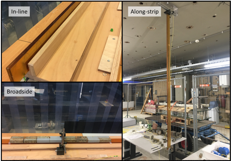
Figure 2.5: Photos of In-line, Broadside and Along-strip loading cases of the Conathane ® strip.
