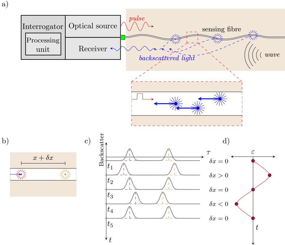
Figure 1.5: Illustration of DAS principle. a) Main components of a DAS system: an optical source sending a pulse into the fibre, and back-scattered light to be captured and processed. b) Two scattering points separated by distance x + \delta x . c) Perturbation of phase of the back-scattered light from the scattering points in (a), to be translated into a strain measurement as in (d).
