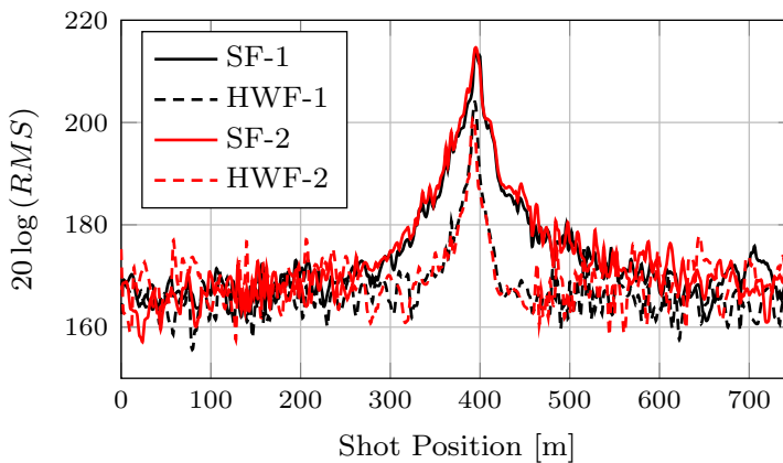
Figure 4.8: RMS amplitudes of Common Receiver Gather at 400 m of four different fibre sections connected to the DAS-Standard system.
