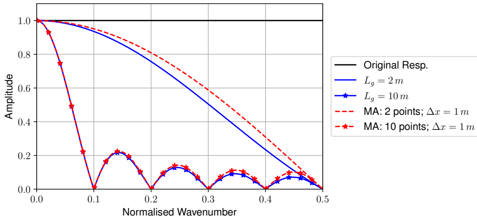
Figure 5.2: Gauge length vs. moving average (MA) wavenumber response
