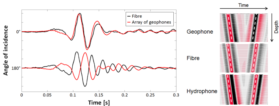
Figure 1.7: Comparison on the polarity of geophone vs. fibre vs. hydrophone ( Dean et al. [2015b]).
