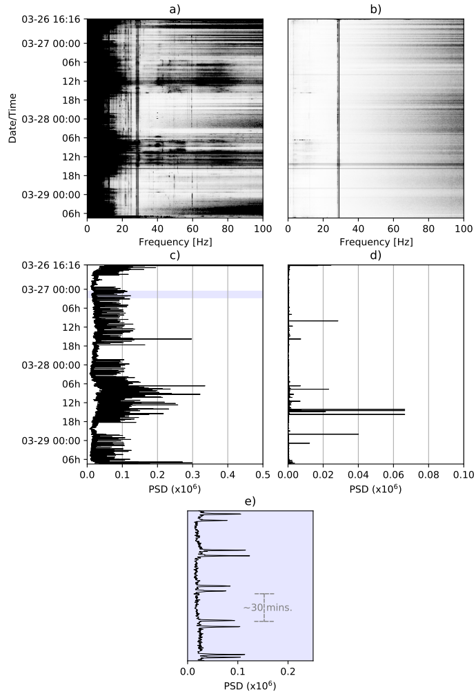
Figure 5.12: Power Spectral Densities (PSDs) of SF data (a) and HWF data (b). PSD summation up to 25 Hz for SF data (c) and HWF data (d) and zoomed view of PSD summation of SF data (e).
