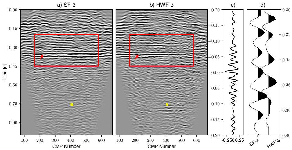
Figure 4.15: CMP-stack comparison between a) SF-3 and b) HWF-3. c) Correlation function between SF-3 and HWF-3. The correlation trace in (c) is calculated from the tapered window of 0.2-0.45 seconds over the CMP range of 165-580. Traces of SF-3 and HWF-3 at CMP-325 (d)
