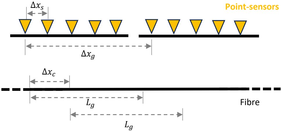
Figure 5.1: Illustration of the gauge length L_g and channel spacing \Delta x_c for continuous/distributed measurements, and equivalent group spacing \Delta x_g and sensor spacing \Delta x_s for point measurements (like geophones).
