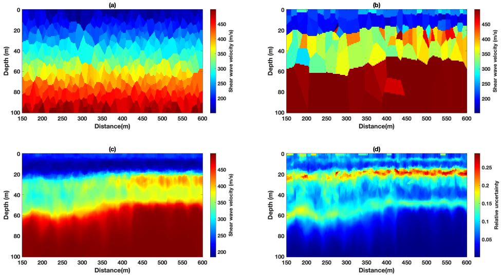
Figure B.4: (a) A random initial model of a chain. (b) The last collected sample of the chain. (c) The posterior mean of the collected samples from 20 parallel chains. (d) The posterior standard deviation of the retained samples.
