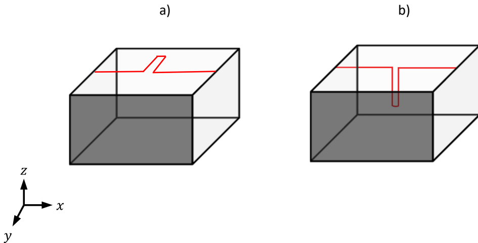
Figure 6.1: Two-component fibre sensors with horizontal in-line and cross-line configuration (a) and a combination of horizontal in-line and vertical configuration (b).
