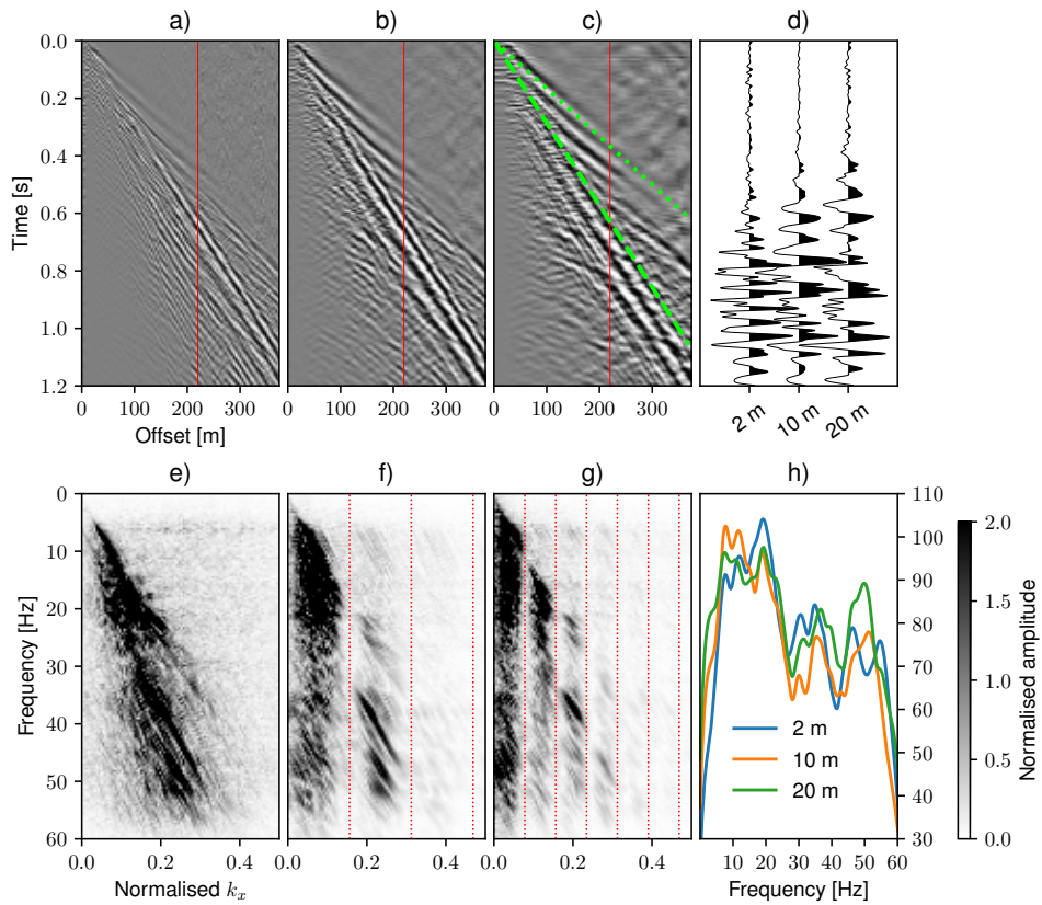
Figure 5.5: SF field data with gauge lengths 2 m (a), 10 m (b) and 20 m (c), and their respective |f, k_x| spectra, 2 m (e), 10 m (f), 20 m (g). Traces at offset 220 m from different gauge lengths (d) and their amplitude spectra in dB scale (h). The red dotted lines in the f and g panels indicate the theoretical positions of the notches at every n/L_g . The green lines in panel c correspond to velocities 350 m/s (dashed) and 600 m/s (dotted).
