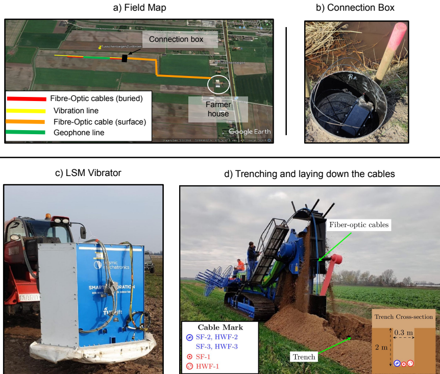
Figure 4.2: Field experiment set-up and components: a) Field map with the position of fibre cables (surface and buried), geophone line and vibration line, i.e. shot positions (survey location: 53^{\circ} 9'16.12''N , 6^{\circ} 50'53.99''E ), b) Connection box with terminations and splices of cables, c) Electrically driven seismic vibrator, based on Linear Motor Technology and d) Trenching and burying fibre-optic cables.
