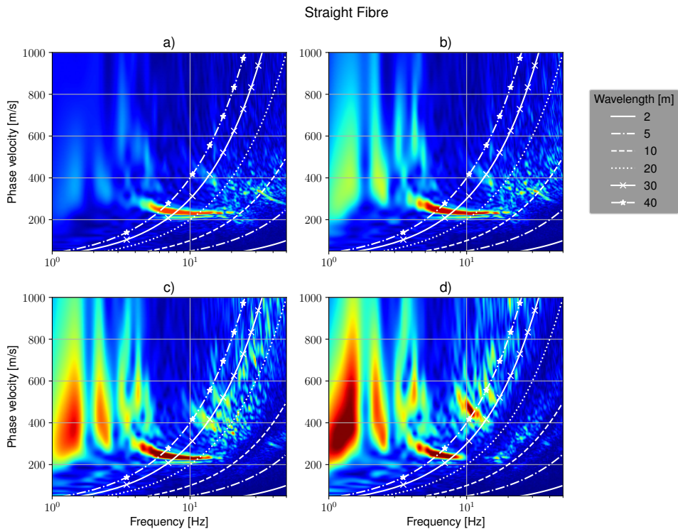
Figure 5.9: SF dispersion images estimated from the field data with different gauge lengths: a) Dispersion image using data with L_g = 2 m, b) L_g = 5 m, c) L_g = 10 m and d) L_g = 20 m.
