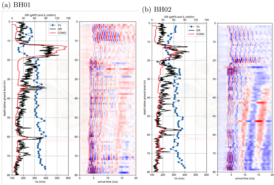
Figure B.8: The measured Induction-Log readings (IL), Gamma Ray (GR), and shear-wave velocity profile ( V_s ) together with the far receiver s-wave seismogram of (a) first borehole (BH01) at x = 220 m and (b) second borehole (BH02) at x = 350 m of the recording line.
