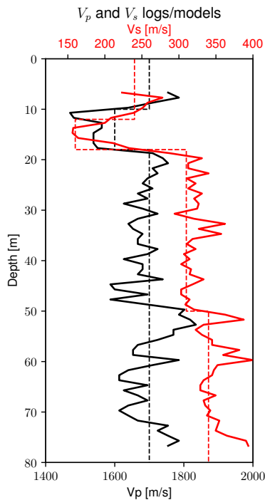
Figure 4.3: P -wave and S -wave velocity logs (solid lines) of the near-surface and models (dashed lines) used for synthetics.
