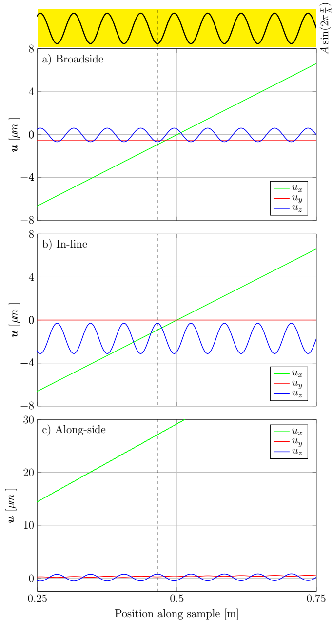
Figure A.2: Displacement field components along the sinusoid A \sin(2\pi \frac{x}{\lambda}) (highlighted by yellow) for loading of 1000 Pa. Zoomed to x=0.25 to x=0.75 m.
