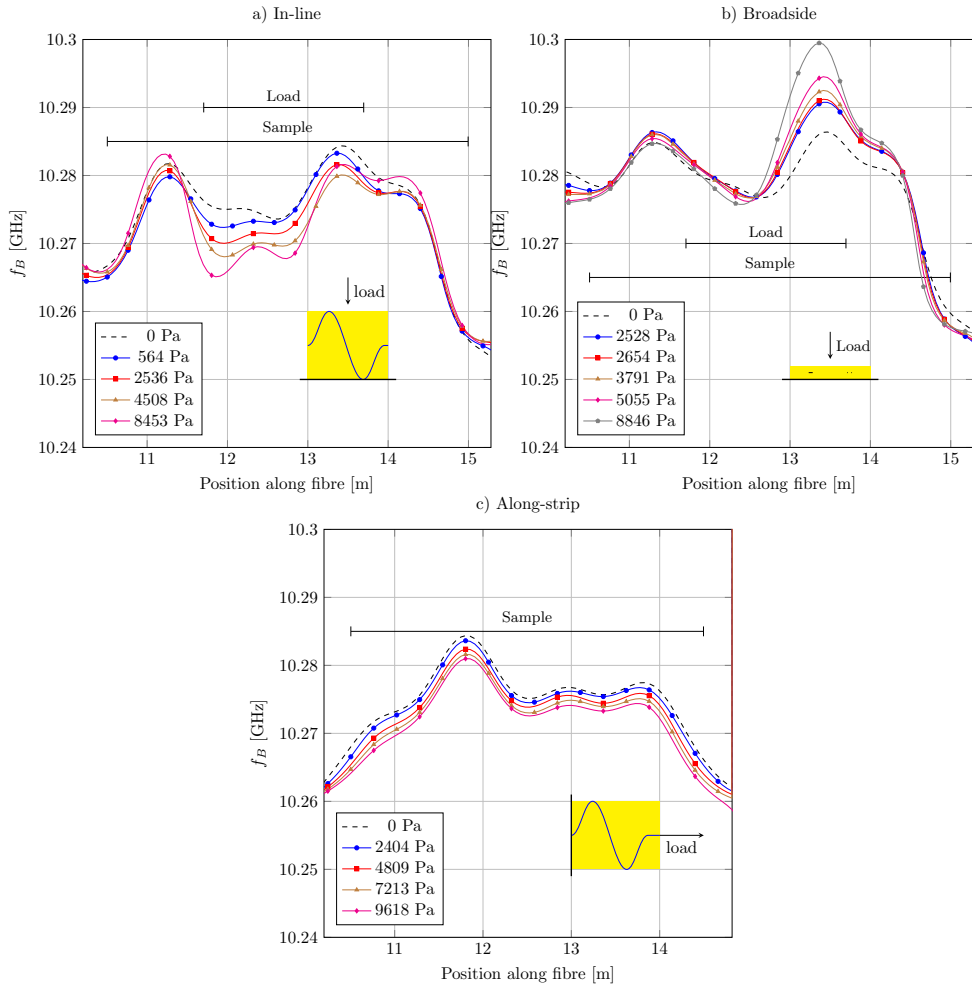
Figure 2.7: Profiles of Brillouin frequency shift for (a) in-line, (b) broadside and (c) along-strip loading.
