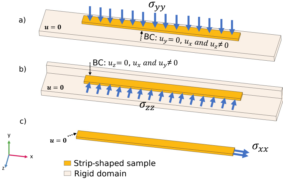
Figure A.1: Loading cases: a) Broadside, b) In-line and c) along-side loading. Note that the boundary load is denoted by the blue arrows and the boundary condition at the contact with a dashed black arrow.
