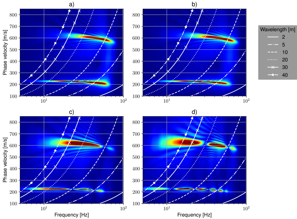
Figure 5.8: Dispersion images estimated from straight fibre synthetic seismograms with different gauge lengths: a) Dispersion image using data with an original sampling of 0.5 m, b) L_g = 2 m, c) L_g = 10 m and d) L_g = 20 m.
