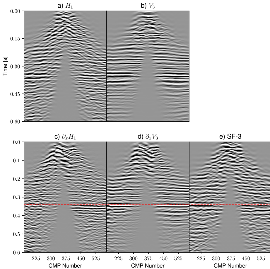
Figure 4.16: CMP-stack sections for a) Geophone H_1 , b) Geophone V_3 , c) (strain-rate) \partial_x H_1 , d) (strain-rate) \partial_x V_3 , and e) SF-3. All images are RMS-normalized and displayed using the same colourmap limits.
