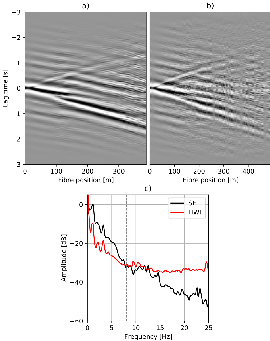
Figure 5.16: Surface wave estimation with crosscorrelation using ambient noise records of 15 hours: virtual shot using SF data (a) and HWF data (b) and their amplitude spectra estimated from the whole shot (c).
