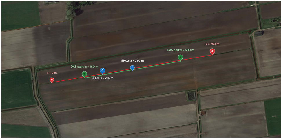
Figure B.5: The acquisition setup of the recorded DAS data in the Groningen area. The red line shows the source line with a length of 750 m and a source spacing of 2 m. The green line shows the DAS straight fiber buried 2 m in depth and with a length of 450 m. The start of the source line is marked as x = 0 and the end of the source line is marked as x = 750 m. The DAS fiber is also located at x = 150 - 600 m. Two boreholes are also drilled to a depth of 80 m at x = 225 m and x = 350 m to measure the shear-wave velocity directly.
