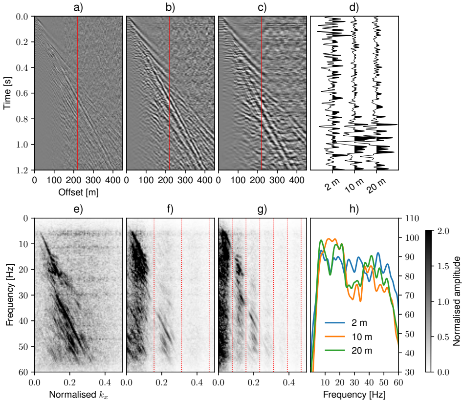
Figure 5.7: HWF ( \alpha = 60^\circ ) field data with gauge lengths 2 m (a), 10 m (b) and 20 m (c), and their respective |f, k_x| spectra, 2 m (e), 10 m (f), 20 m (g). Traces at offset 220 m from different gauge lengths (d) and their amplitude spectra in dB scale (h). The red dotted lines in f and g panels indicate the theoretical positions of the notches at every n/L_g .
