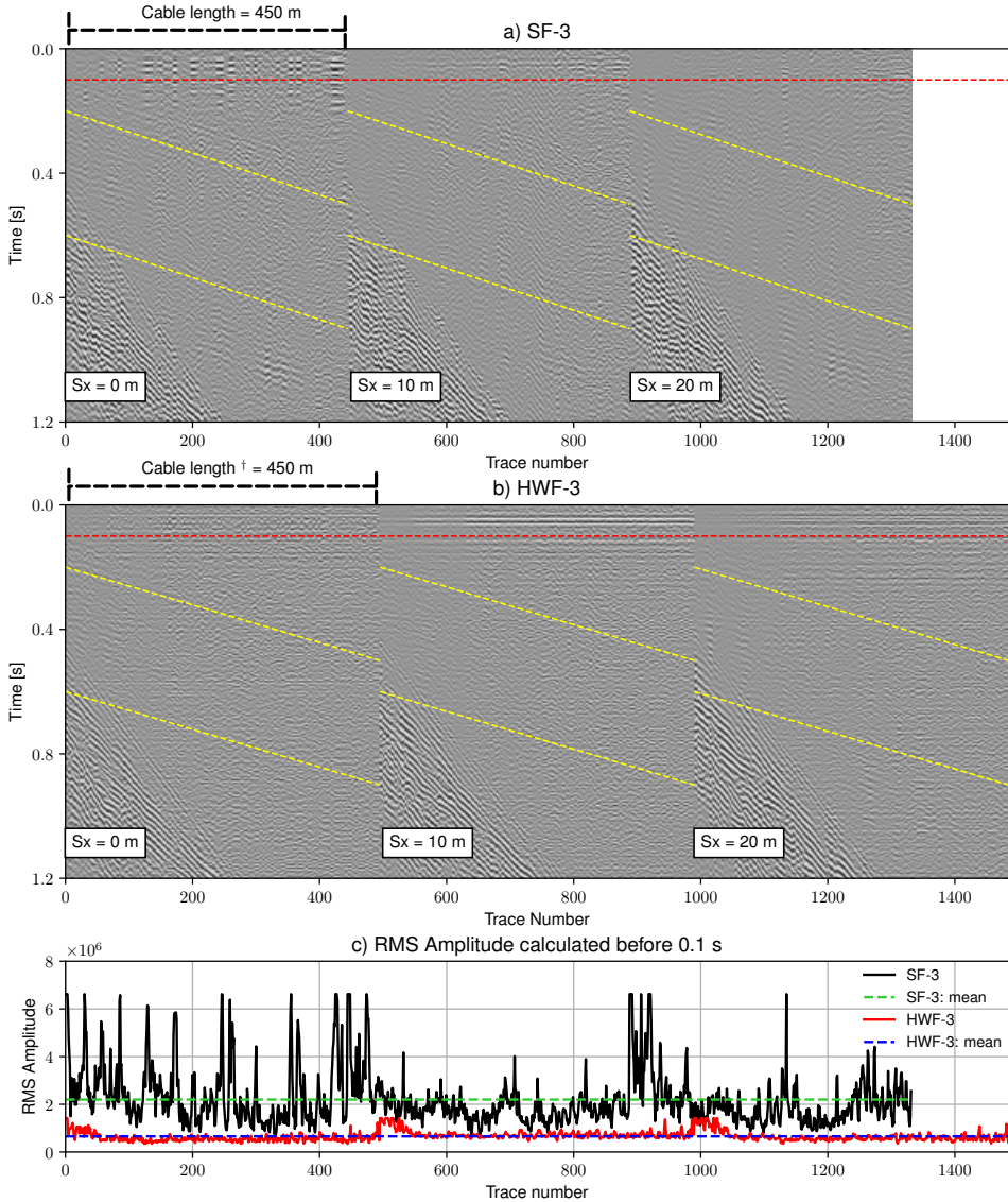
Figure 4.12: Common-shot gathers at positions 0, 10 and 20 m for SF-3 (a) and HWF-3(b), and c) RMS amplitude calculated before 0.1 s. † Cable length \neq fibre length.
