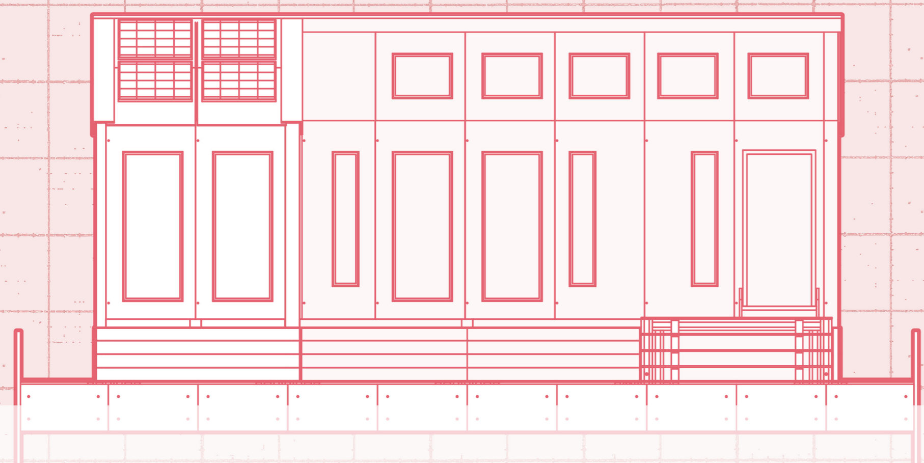
South Elevation | 1:100
