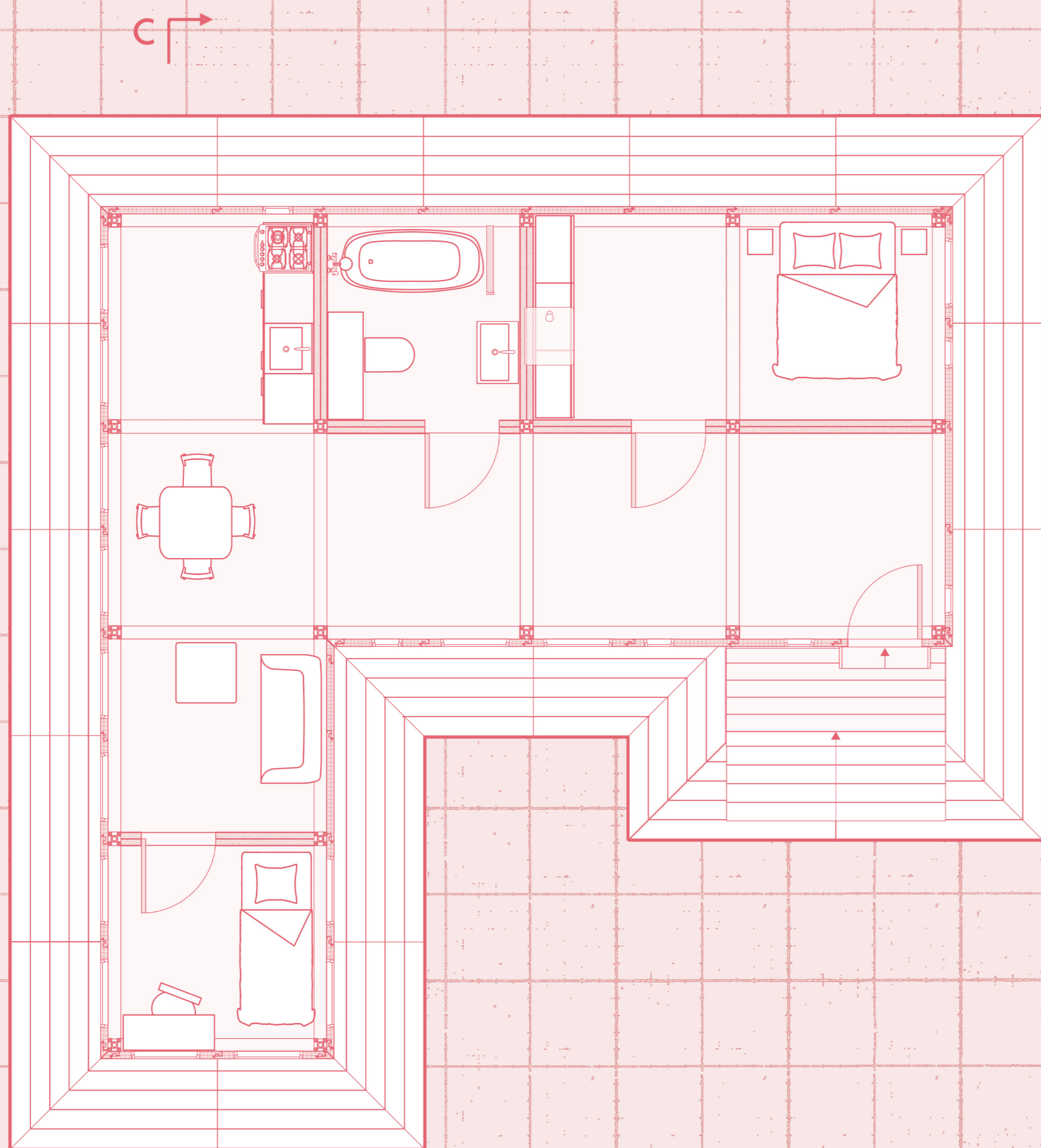
Floor Plan | 1:100
