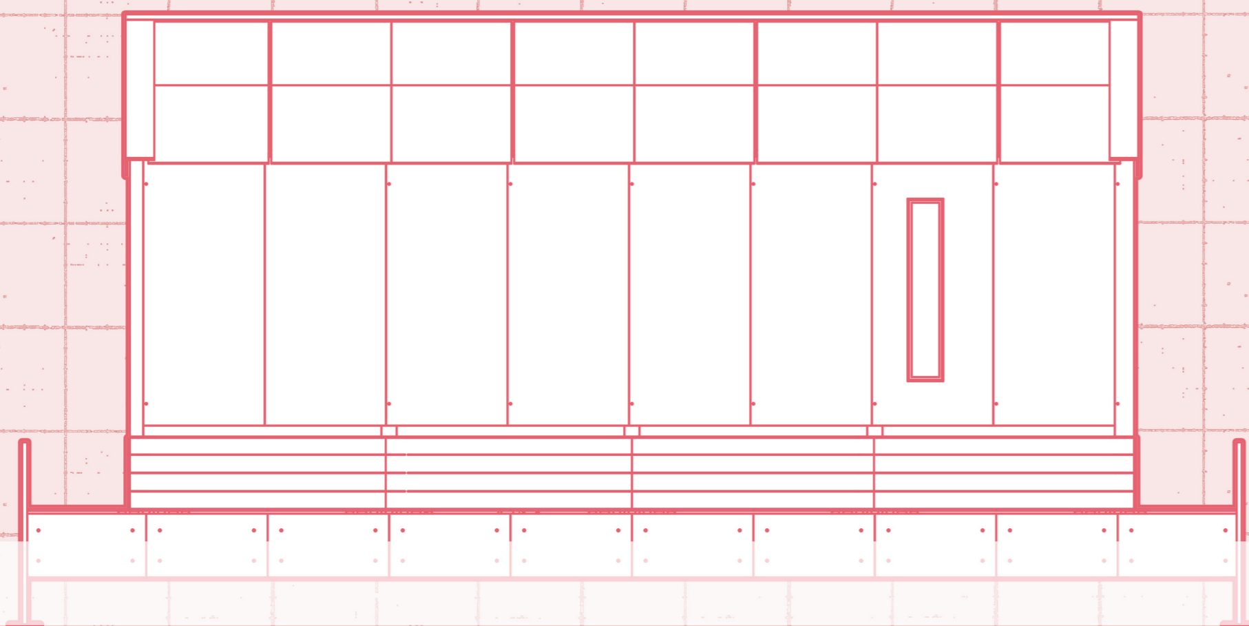
North Elevation | 1:100
