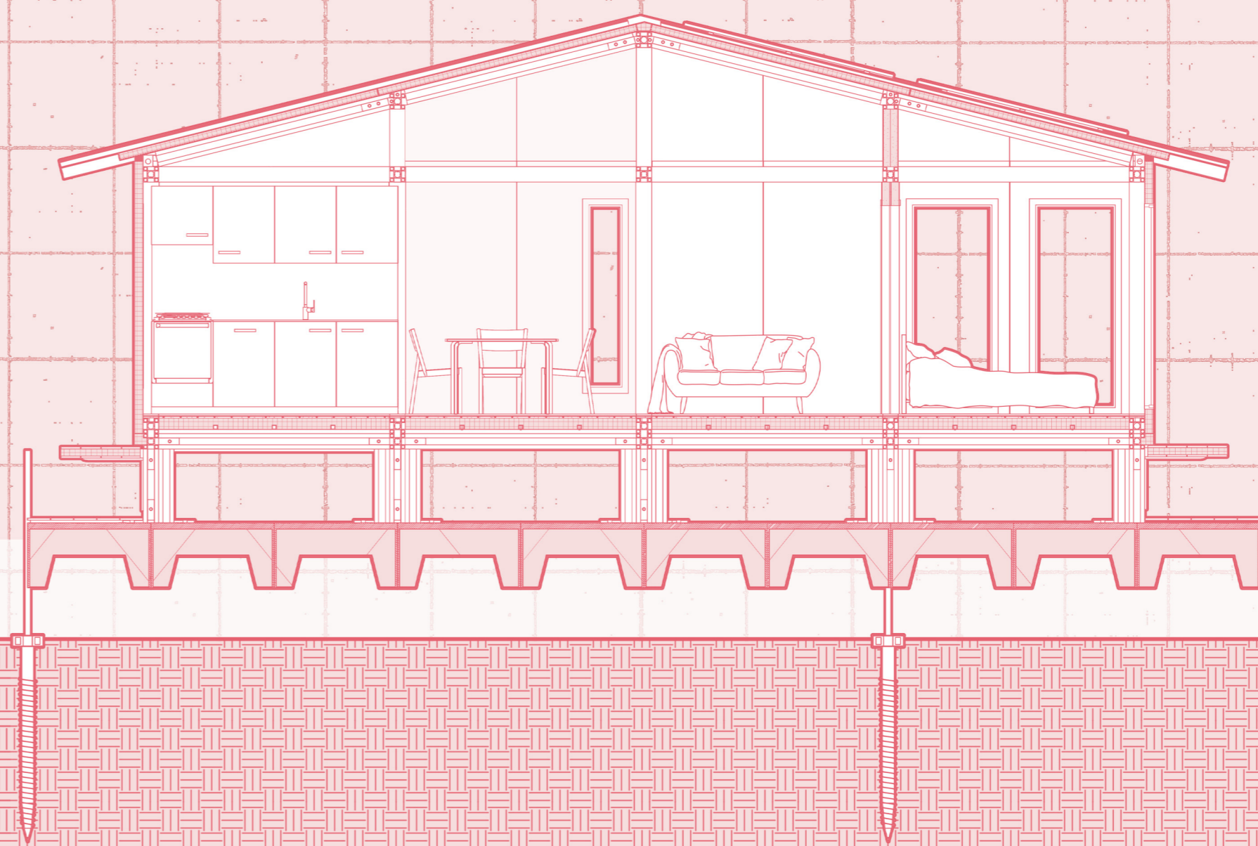
Section CC' (open deck) | 1:100
