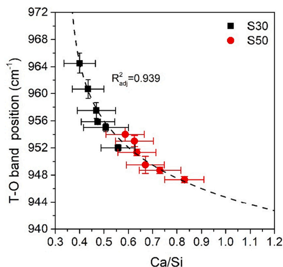
Fig. 15. Correlations of Ca/Si ratio of C-(N-)A-S-H gel as main reaction product and the position of main T-O vibration band in FTIR.
