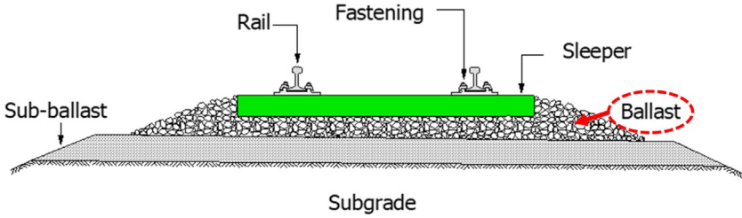
Fig. 14.1 Conventional ballast track.
