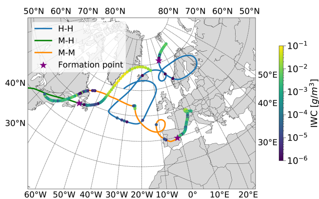
Figure 4. IWC (colour coded) along three example trajectories from the cirrus classifications of formation and measurement at high latitudes (H–H, blue); formation at mid-latitudes and measurement at high latitudes (M–H, green); and formation and measurement at mid-latitudes (M–M, orange). The formation point is indicated with a purple star.
