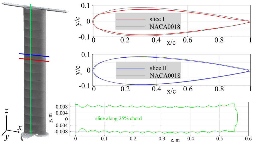
Figure 5.2: Visualization of the outer shape scan results of the Delft-Pazy wing
