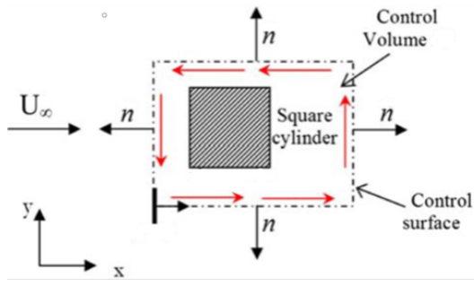
(a) control volume around a square cylinder
