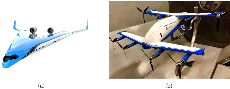
Figure 1.1: (a) Flying V concept airplane (image credit: Edwin Wallet), (b) LA-8 eVTOL testbed in the wind tunnel at NASA Langley (from North et al., 2021)
