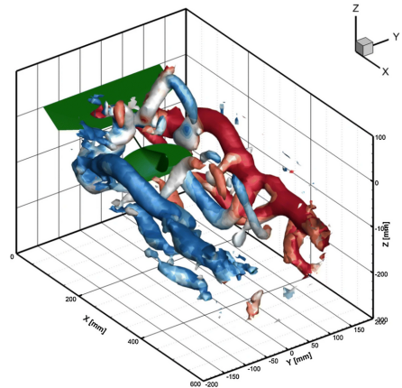
(b) isocontours of the measured vorticity
