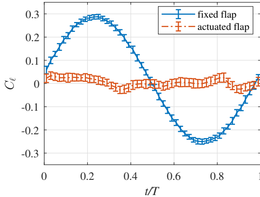
Figure 3.3: Phase-averaged lift coefficient over the period for the pitching wing with fixed and actuated flap
