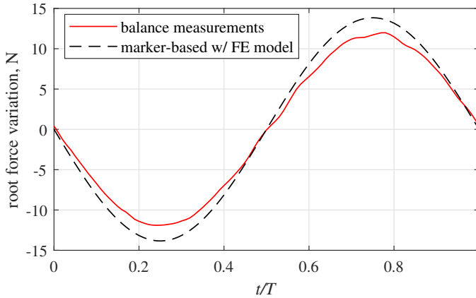
Figure 4.12: Comparison of the root shear force from the FE model with the balance measurements
