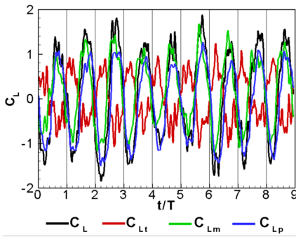
(b) unsteady lift coefficient
