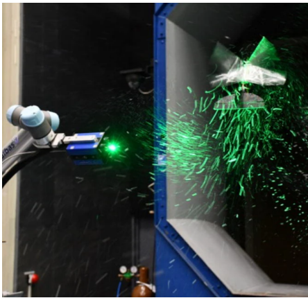
(a) robotic PIV measurement in the wind tunnel
