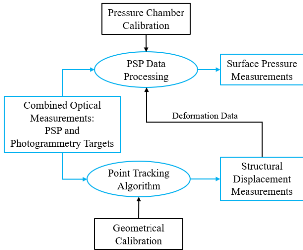
(a) combined measurement approach with PSP and point tracking
