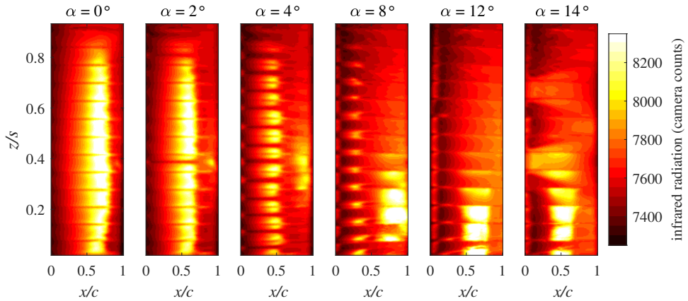
Figure 5.18: Infrared thermography images of the Delft-Pazy wing for 0^\circ \leq \alpha \leq 14^\circ
