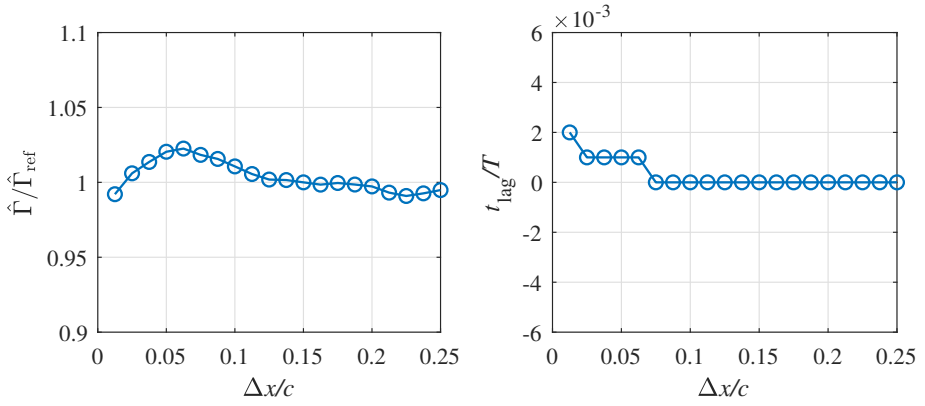
(a) variation of the upstream segment of the integration path
