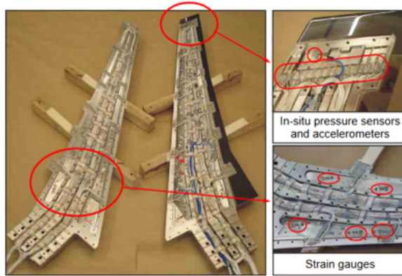
Figure 1.5: Heavily instrumented wing model for wind tunnel testing, from Ballmann et al. (2008)
