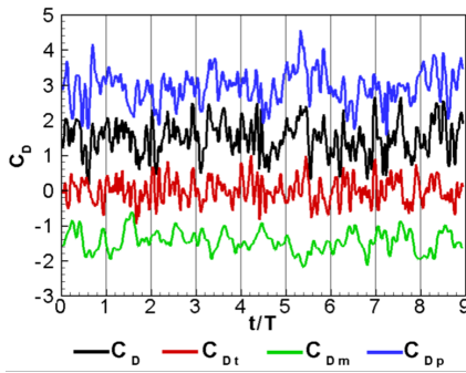
(c) unsteady drag coefficient
