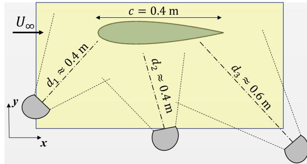
Figure 3.4: Sketch of the three CVV positions with respect to the wing and the illuminated volume
