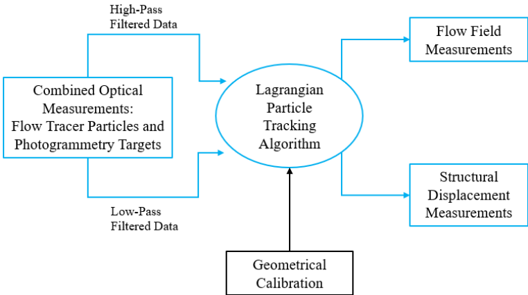
(b) integrated measurement approach with LPT and point tracking (used in this thesis)
