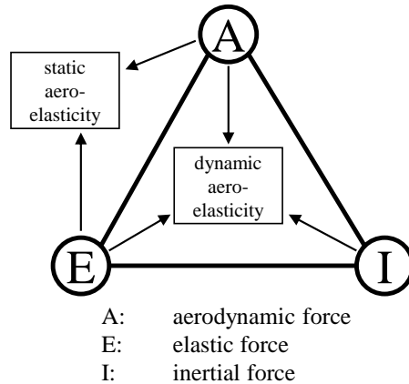
Figure 1.4: Illustration of Collar's triangle of forces
