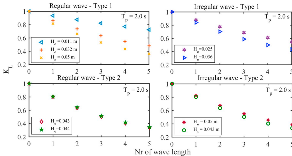
Fig. 5. Effective wave transmission K_L in cases of sparse vegetation, wave period of 2s, different wave height.
