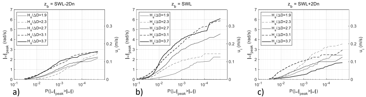
Figure 12: Probability of exceedance (per wave and unit) of peak rocking angular impact velocity. Graphs are given for three z_b , and each wave condition. The right axis gives the impact velocity of the upper leg derived by eq. (3).
