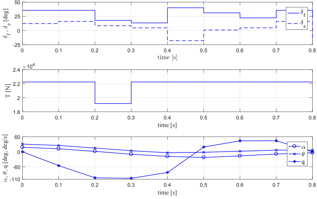
Fig. 20 Control input variation and state trajectory initialized at (\alpha, \theta, q) = (18 \frac{\pi}{180} \text{ rad}, 31 \frac{\pi}{180} \text{ rad}, 0 \text{ rad/s}) at Mach 0.4, sea level – Monte Carlo analysis for backward reachable set, nominal Cessna Citation II
