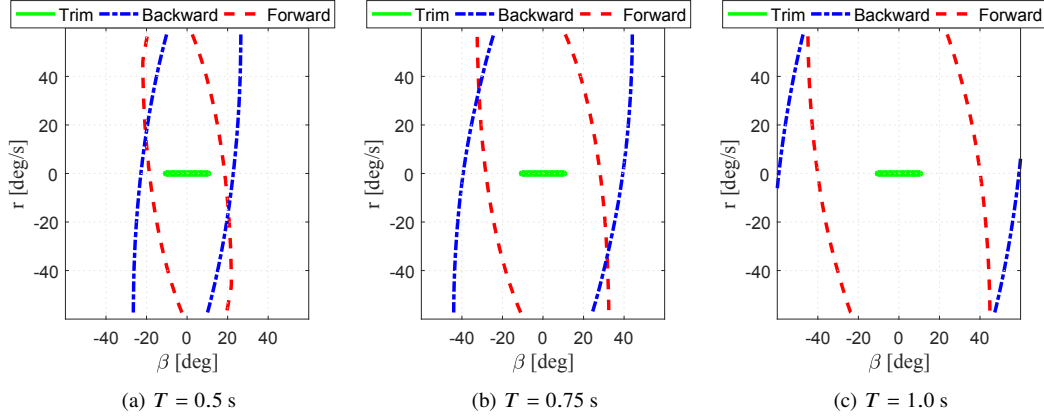
Fig. 28 Lateral safe flight envelope for nominal Cessna Citation II at Mach 0.4, sea level (variation with time horizon)
