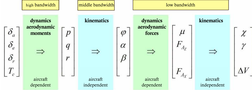
Fig. 5 Time scale separation of aircraft dynamics [27]
