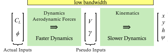
Fig. 4 Time scale separation implemented by Kitsios and Lygeros [10]
