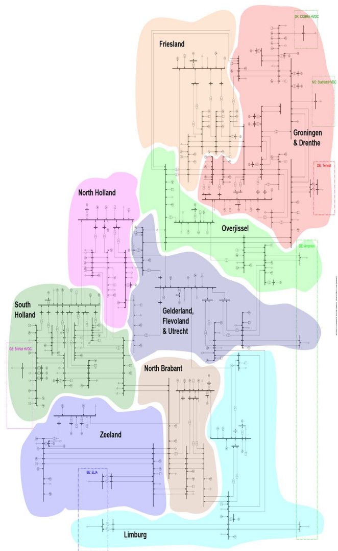
Fig. 2. Division of the single line diagram into geographical zones.
