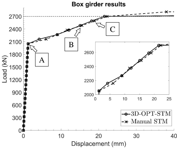
Figure 4.20: Load-displacement results of the 3D-OPT-STM design and classic STM design of the box girder.
