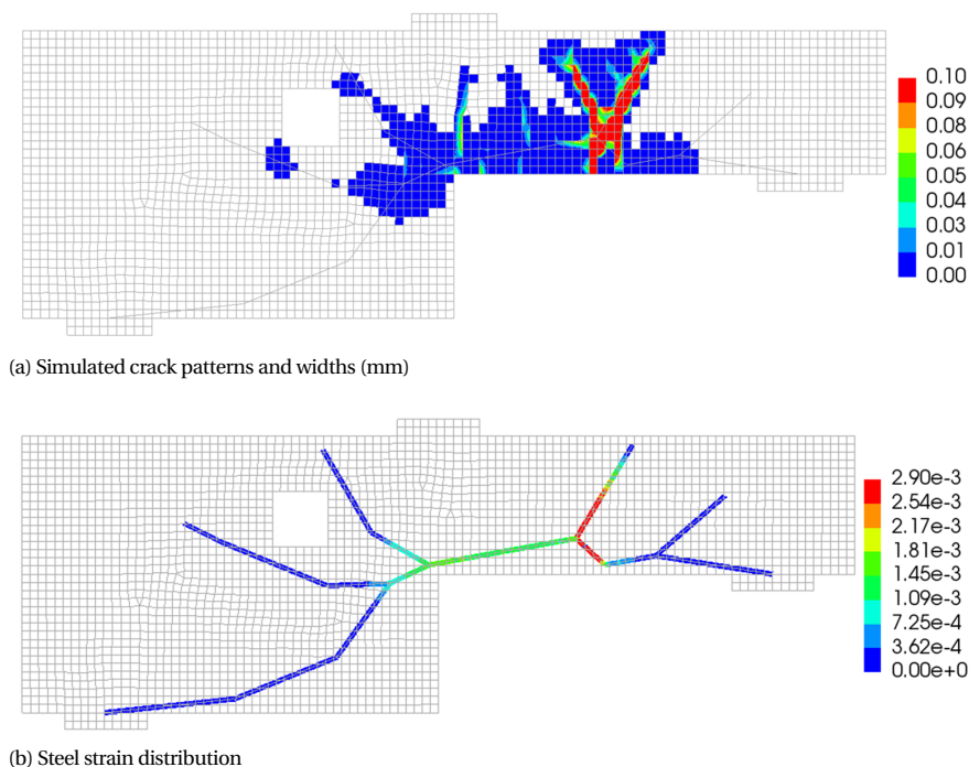
Figure 3.32: Structural response of the uncorrected truss-like structure in the ultimate state.
