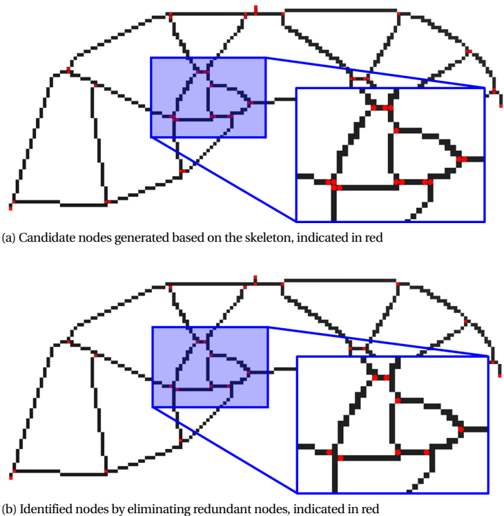
Figure 3.7: Node identification of the truss-like structure.
