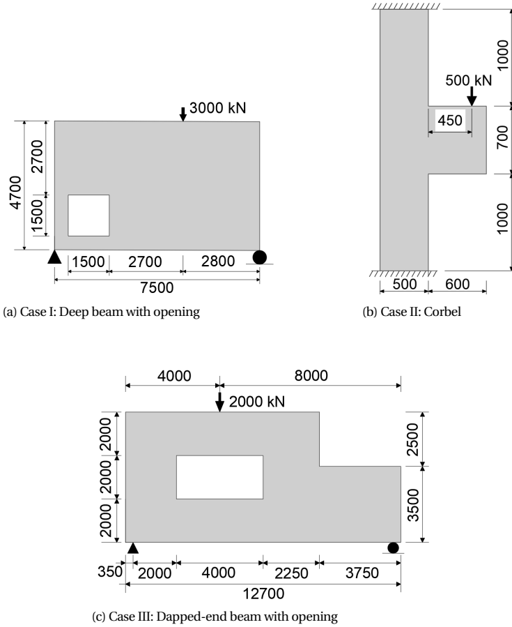
Figure 2.15: Basic information of three cases (mm)
