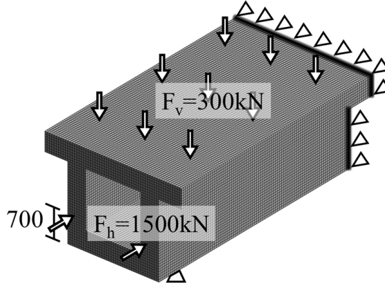
(a) Box girder problem
