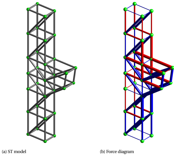
Figure 4.13: The manually created ST model of the corbel. Red and blue bars indicate tensile and compressive members respectively. The bar width indicates the force magnitude.
