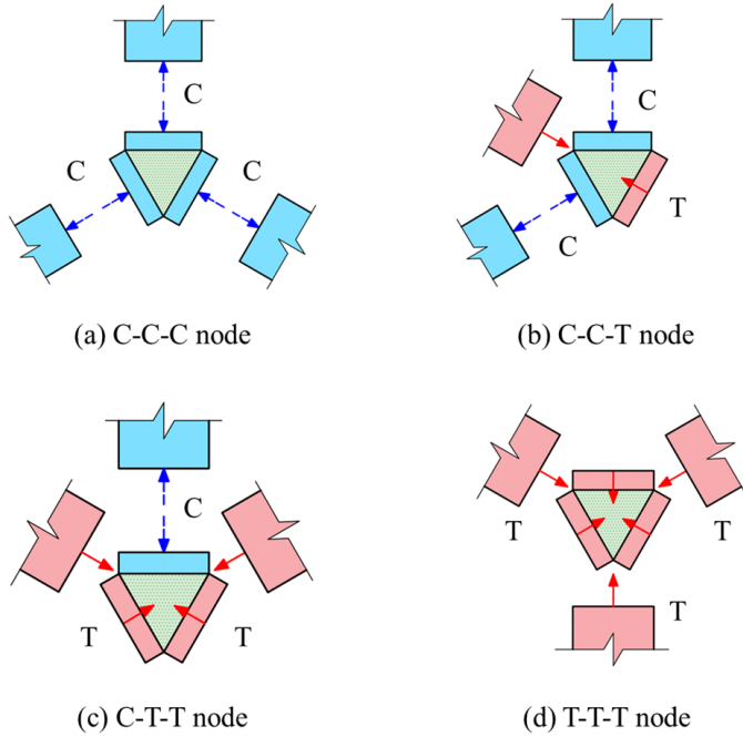
Figure 1.3: Four types of nodal zones in 2D ST models. Blue regions and red regions indicate struts and ties respectively. Green regions indicates nodal zones. T indicates forces in tensile ties, whereas C indicates force in compressive struts. All the nodes are in the compressive stress state and they are categorized based on the original forces.
