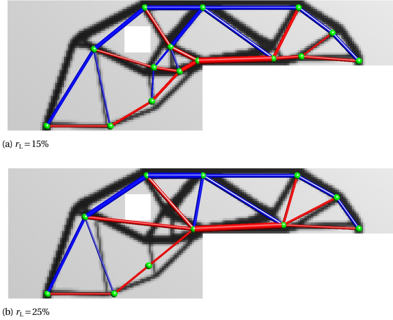
Figure 3.28: Generated OPT-STM with two merging lengths. Black pixels present the TO result. The blue and red lines indicate struts and ties respectively. The line width indicates the magnitude of axial forces.
