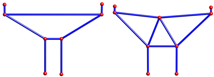
(a) Single-load result using the load combination where Load-1 and Load-2 act simultaneously (b) Multi-load result using all three load combinations
