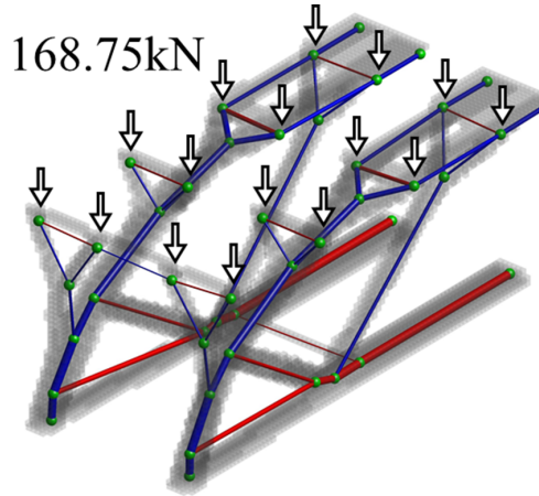
(b) 4 \times 4 loads
