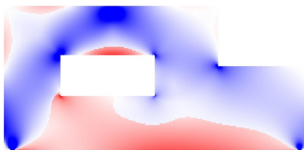
(c) Case III: Dapped-end beam with opening (mesh size: 50 mm)
