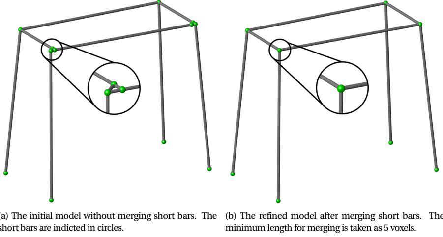
Figure 4.4: The generated truss-like models generated by the proposed extraction process based on the table-like model (see in Figure 4.2)
