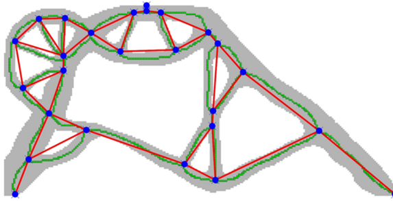
Figure 2.9: Obtained truss-like structure. The grey part is the binary TO result, the green pixels form the thinned skeleton, blue points and red lines are the identified nodes and members respectively.
