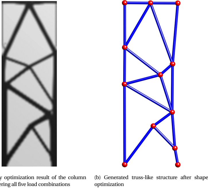
Figure 5.9: Multi-load results for the column case
