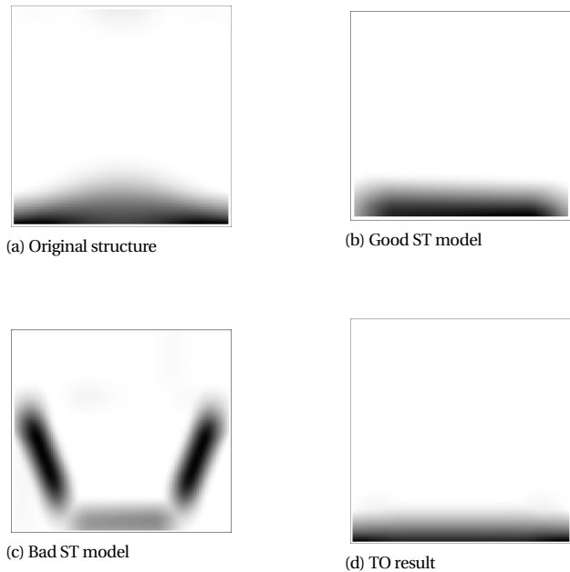
Figure 2.14: Scaled tensile principal stress after non-local averaging
