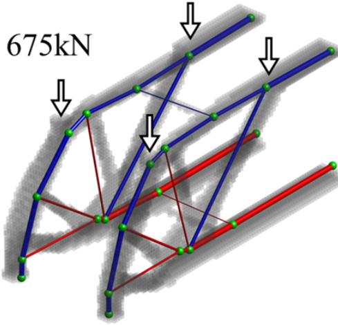
(a) 2 \times 2 loads
