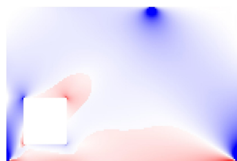
(a) Case I: Deep beam with opening (mesh size: 50 mm)
