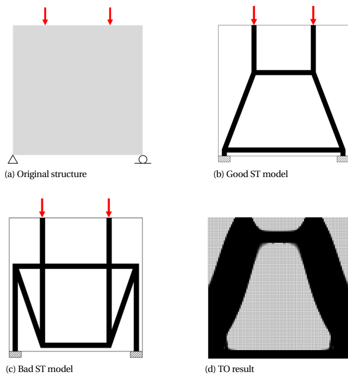
Figure 2.11: Geometries considered to illustrate the evaluation method. (a) shows the deep beam design problem; (b) and (c) show manually generated ST models; (d) shows the TO result.
