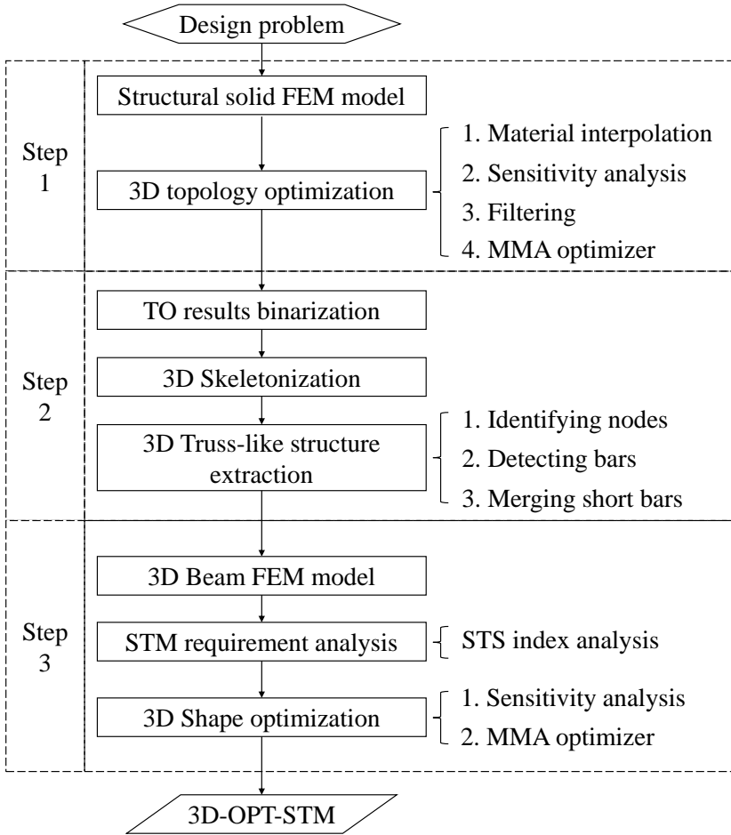
Figure 4.1: Flowchart of the 3D-OPT-STM generation method
