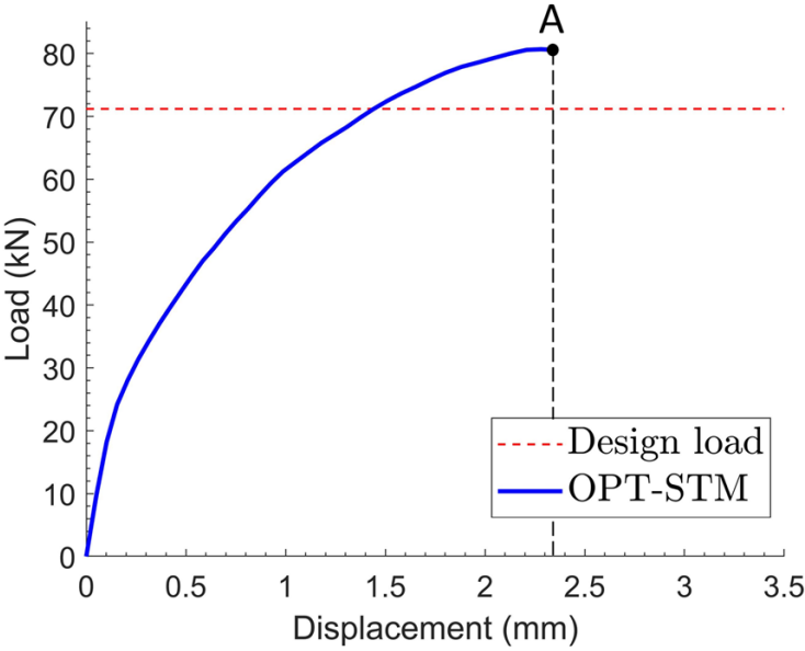
Figure 3.24: Load-displacement curve of the OPT-STM based design.
