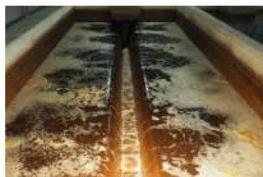
(a) Full-scale RSF during collapse pulsing 40 m/h backwashing scour
