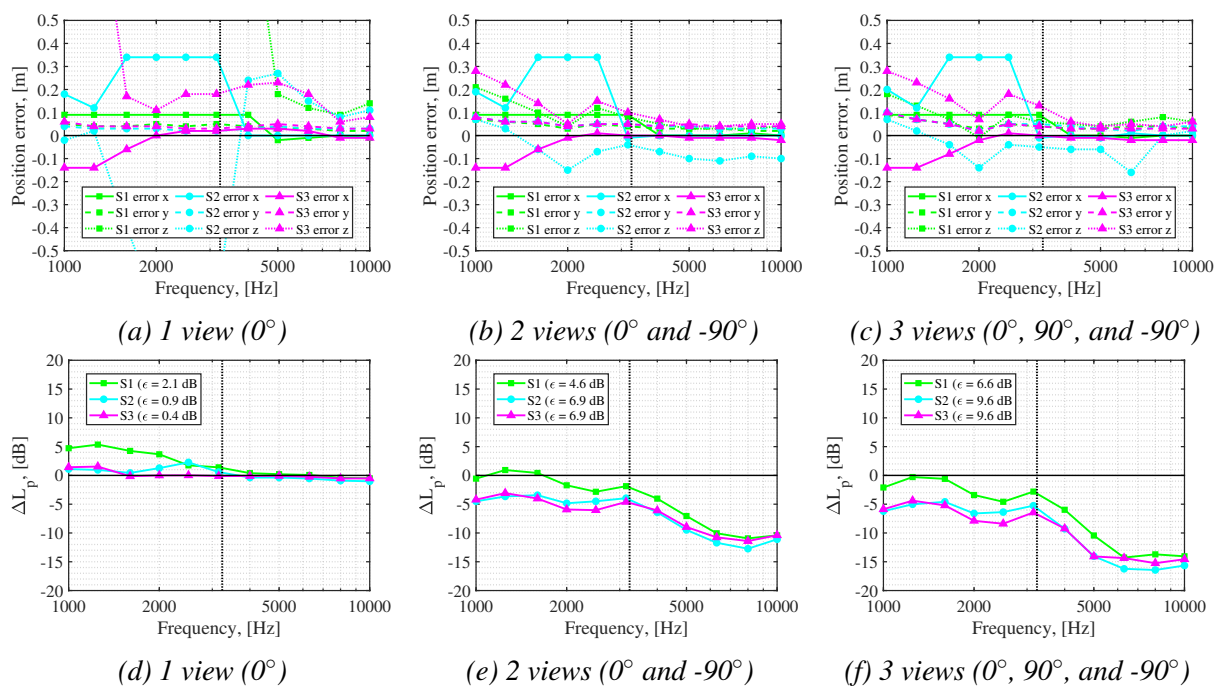
Figure 4: Relative errors in position in x , y , and z (first row) and L_p (second row) for each speaker made by CFDBF. The vertical dotted line represents the Rayleigh resolution limit.
