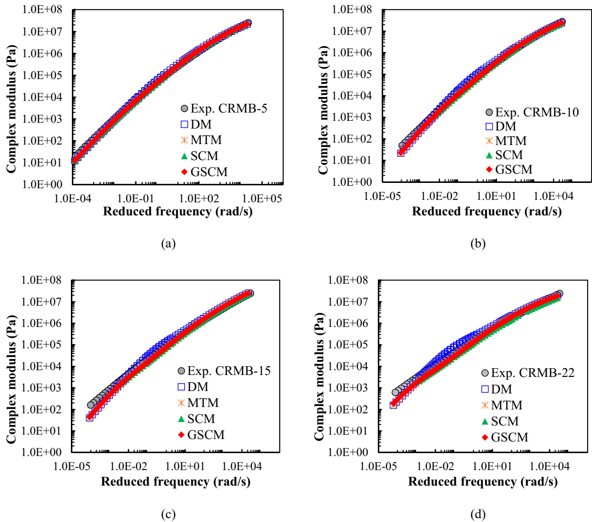
Fig. 12. Micromechanical model predicted complex moduli of CRMB using the calibrated constituent parameters.
