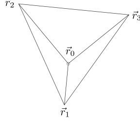
Figure A.1: Representation of a triangle.
