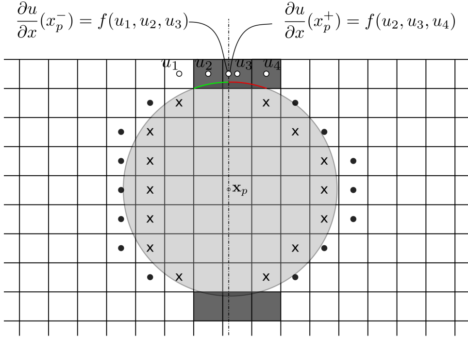
Figure 10: Representation of the missed cells and the shear rate computation in those cells.
