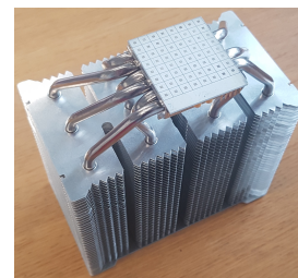
Fig. 1. State-of-the-art fabricated chip-integrated array with the Mugen MAX fanless CPU heatsink [14] (picture taken from [9]).
