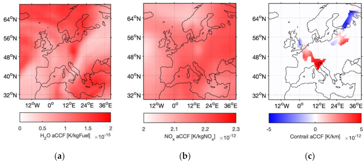
Figure 1. Algorithmic climate change functions for \text{H}_2\text{O} (a), \text{NO}_x (b), and contrails (c) on 18 December 2015, 6.00 p.m. UTC as function of latitude and longitude on flight level 390.
