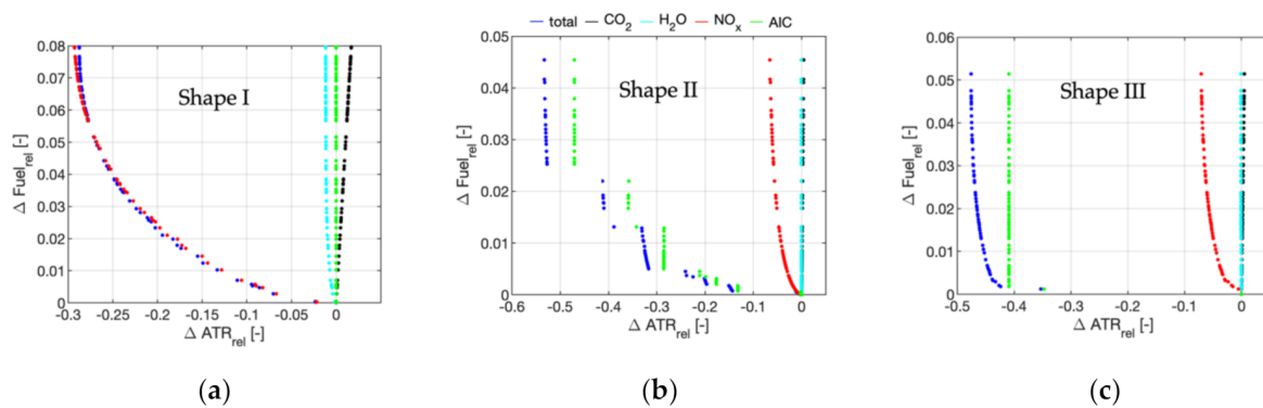
Figure 6. Pareto fronts for Baku–Luxembourg (a), Luleå–Gran Canaria (b), and Helsinki–Gran Canaria (c). The colored dots indicate the individual contribution of CO 2 (black), H 2 O (cyan), NO x (red), and contrails (green) to the overall climate impact reduction (blue) for a given fuel increase. Results are expressed relative to the fuel burn and the total climate impact of the minimum fuel case.
