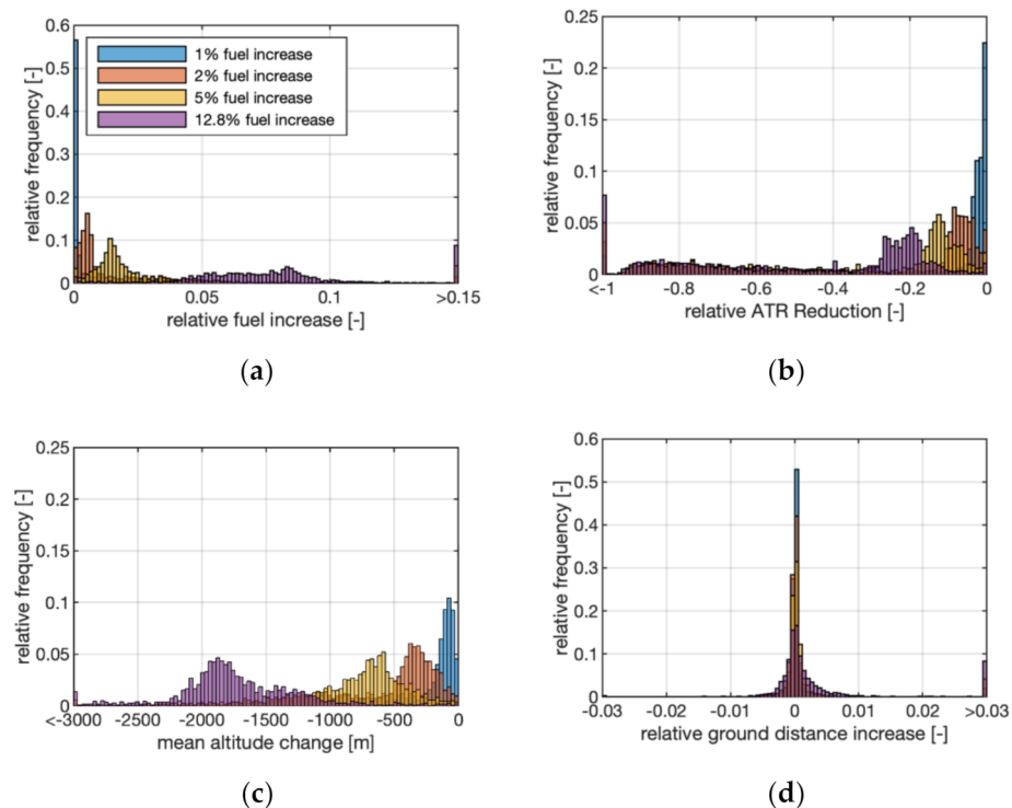
Figure 9. Frequency distributions of the relative fuel increase (a), the relative ATR reduction (b), the mean altitude change (c), and the relative ground distance increase (d) compared to the minimum fuel trajectory based on the top 2000 routes for 1% (blue), 2% (orange), 5% (yellow), and 12.8% (purple) overall fuel penalty.
