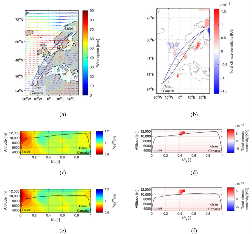
Figure 5. Optimized trajectories for the route Luleå-Gran Canaria. The lateral path of the minimum fuel trajectory (black) is illustrated including the wind situation (a) and the total climate sensitivity (b) at an average altitude of 10,686 m. The orthodrome is depicted in blue. The lateral path of the minimum climate impact trajectory is not shown separately, since only minor deviations from the minimum fuel trajectory occur. Altitude profiles along the cross section of the lateral path are shown for the minimum fuel case (c), (d) and the minimum climate impact case (e), (f) as a function of the relative flight time t/t_f . The wind situation for the vertical trajectories is indicated as ratio between ground speed v_{GS} and true airspeed v_{TAS} . Values greater than one indicate tailwind areas, values smaller than one indicate headwind areas.
