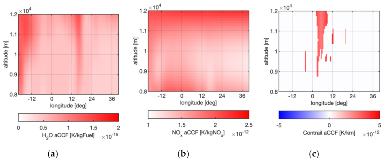
Figure 2. Algorithmic climate change functions for \text{H}_2\text{O} (a), \text{NO}_x (b), and contrails (c) on 18 December 2015, 6.00 p.m. UTC as function of longitude and altitude at 48^\circ \text{N} .
