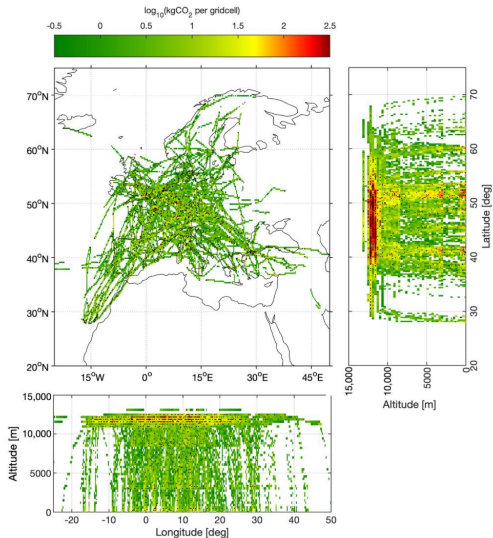
Figure 4. Cumulative CO 2 emission distributions of the chosen reference traffic on 18 December 2015, between 11.30 a.m. and 12.00 p.m. UTC as function of latitude and longitude (top left), altitude and latitude (top right) as well as altitude and longitude (bottom). Black dots indicate aircraft positions at 12.00 pm UTC.
