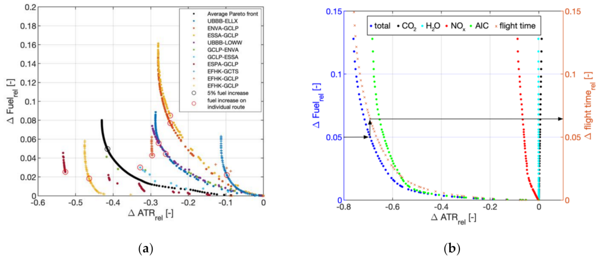
Figure 7. Top 10 single route Pareto fronts and corresponding average Pareto front (a) and average Pareto front (b) for the top 2000 routes with individual contribution of the species CO 2 (black), H 2 O (cyan), NO x (red), and contrails (green) to the overall climate impact reduction (blue) for a given fuel increase. Results are expressed relative to the minimum fuel case.
