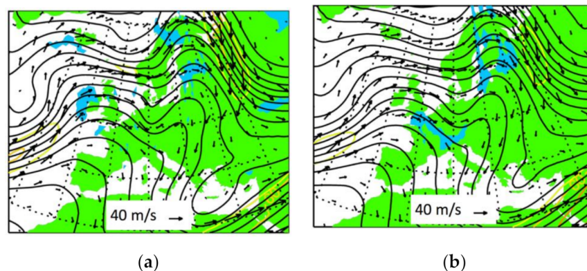
Figure 3. Geopotential height (black contours), wind situation (arrows), and regions of potential contrail formation (blue) over Europe on 18 December 2015, 12.00 p.m. UTC based on European Centre for Medium-Range Weather Forecasts (ECMWF) ERA-Interim re-analysis data on pressure levels 250 hPa (a) and 200 hPa (b).
