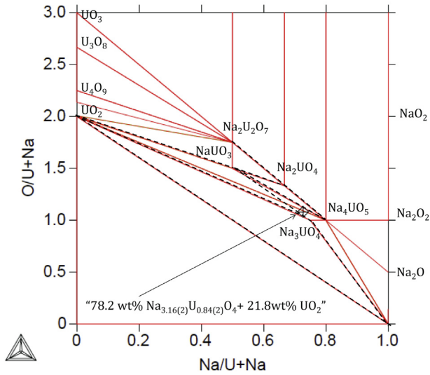
Fig. 12. Calculated Na-U-O phase diagram at 900 K and 1 bar (red line), and comparison with the phase boundaries the ternary phase fields as suggested by [9] (black dotted line). (For interpretation of the references to colour in this figure legend, the reader is referred to the web version of this article.)
