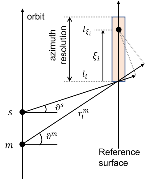
Fig. 2. (a) Phase term due to the azimuth sub-pixel position \xi_i . The signal path length changes because of the variation in squint angle \vartheta , resulting in a phase term \phi_{i,\xi} . Adapted from Marinkovic et al. (2004). (b) Sub-pixel phase term in azimuth as a function of the dominant scatterer location and \Delta f_{DC} in case of Radarsat-2.
