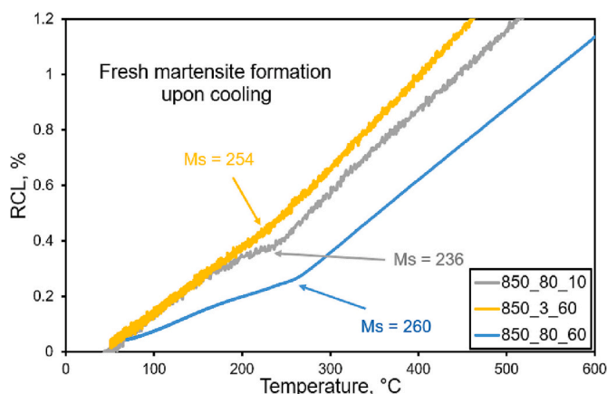
Fig. 4. The dilatometric curves registered during cooling at various rates after second step of intercritical annealing at 850 °C; M_s = 260 °C (blue); M_s = 254 °C (yellow); M_s = 236 °C (grey). (For interpretation of the references to colour in this figure legend, the reader is referred to the web version of this article).
