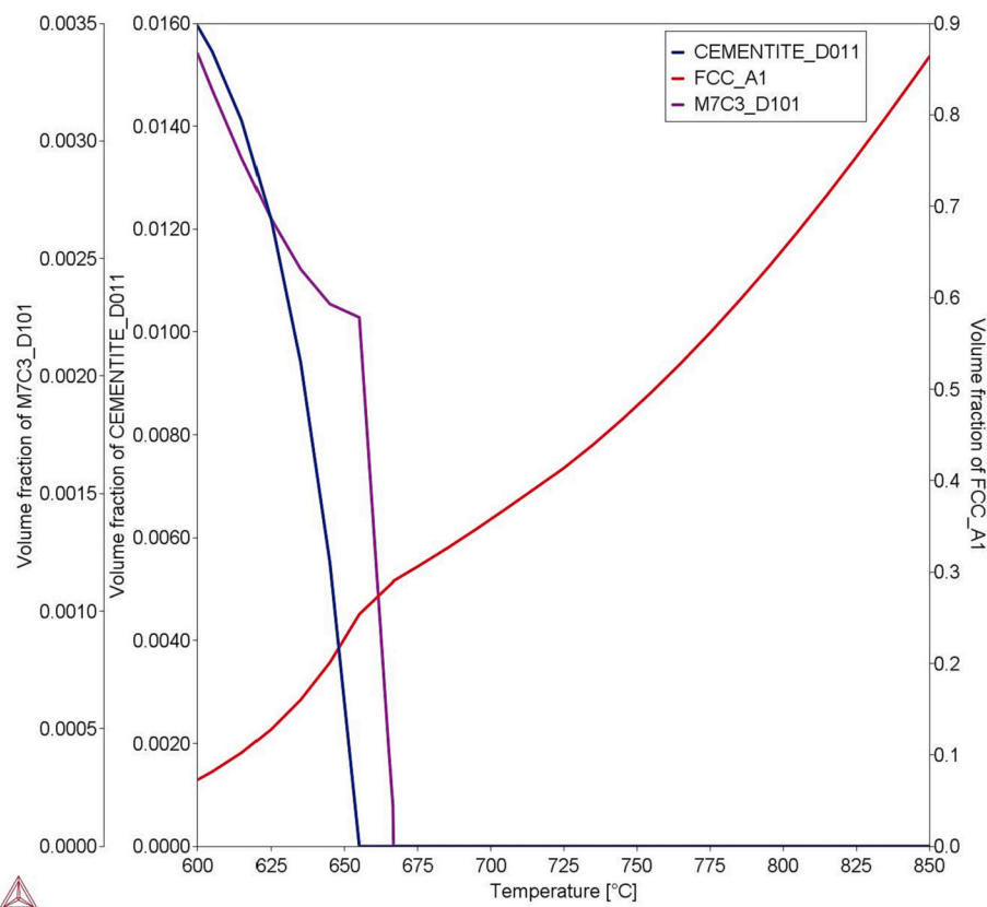
Fig. 7. Change in the fractions of austenite, cementite and \text{M}_7\text{C}_3 carbides in the annealing temperature range from 600 °C to 850 °C.
