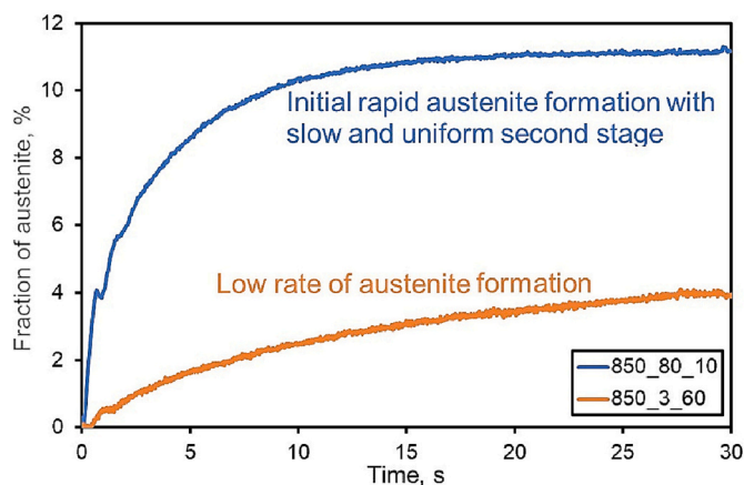
Fig. 3. The kinetics of austenite formation during the second step of intercritical annealing at 850 °C. Specimens heated and cooled at rates of: 80 °C/s and 10 °C/s (blue), 3 °C/s and 60 °C/s (orange), respectively. (For interpretation of the references to colour in this figure legend, the reader is referred to the web version of this article).
