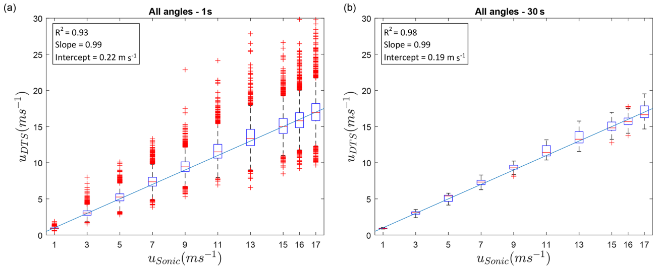
Figure B2. Comparison of AHFO and sonic anemometer wind speed, combining all angles of attack at a 1 s (a) and 30 s (b) resolution; n_{\text{space}} = 10 , n_{\text{time}} = 1 and 30. The line represents the 1 : 1 line.
