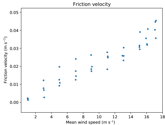
Figure C1. Friction velocity ( \text{m s}^{-1} ) in the wind tunnel during the AHFO experiment.
