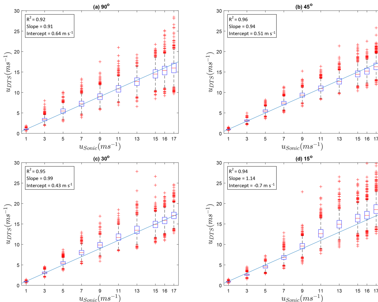
Figure B1. Comparison of AHFO and sonic anemometer wind speed at a 1 s temporal resolution for the four different angles of attack: (a) 90°, (b) 45°, (c) 30° and (d) 15°; n_{space} = 10 , n_{time} = 1 . The line represents the 1 : 1 line.
