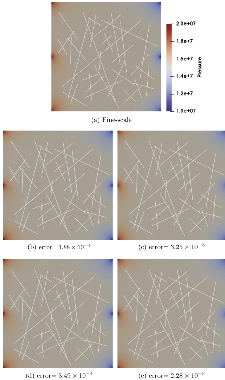
Fig. 12. Pressure plots for 2D F-ADM test case. Shown are the fine-scale solution (a), decoupled F-ADM with thresholds 0.1 (b) and 0.8 (c), and coupled F-ADM with thresholds 0.1 (d) and 0.8 (e), respectively.
