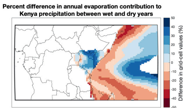
FIG. 5. The difference between the driest and wettest years of evaporation contribution to Kenyan precipitation.
