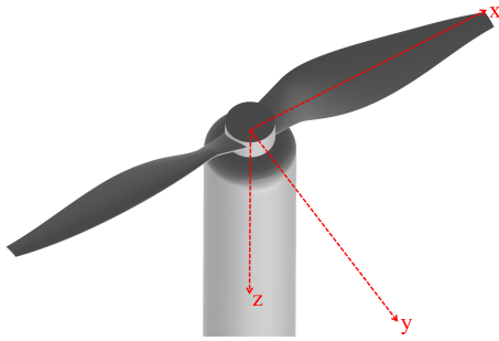
Figure 4. Propeller geometry and reference system.
