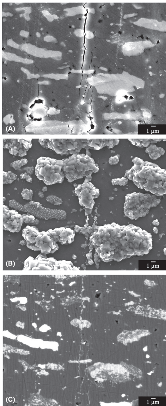
FIGURE 11 SEM images of the same crack area before and after heating at 1000°C for 1 h in air. A, Before oxidation. B, After oxidation and before polishing. C, Polished surface showing fully filled cracks
