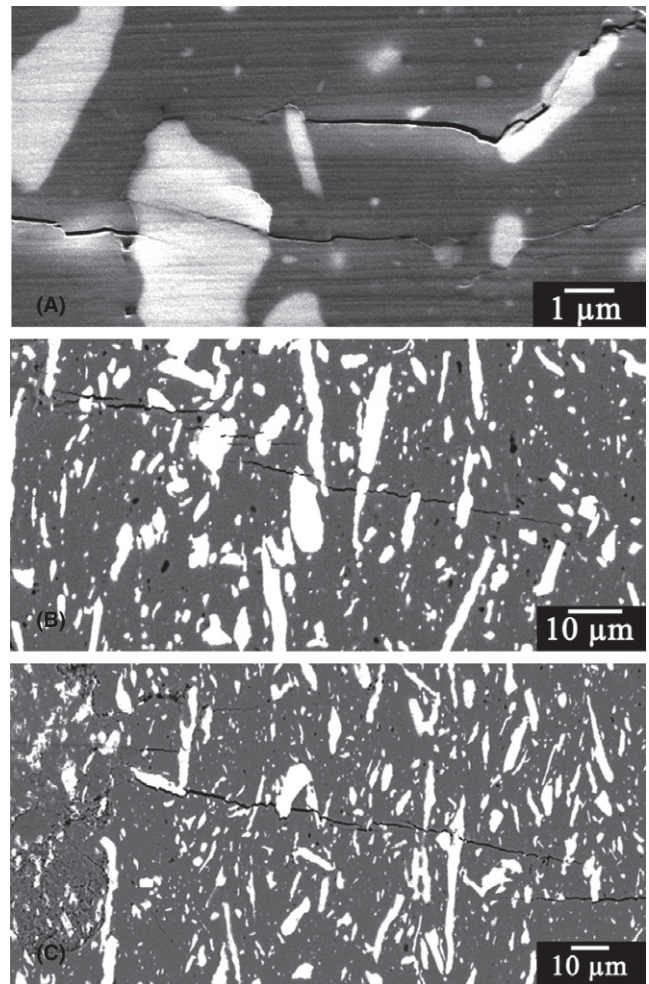
FIGURE 8 Toughness enhancement mechanisms of Ti 2 AlC in Al 2 O 3 . SEM images (A) cracks blunted by particle, (B) and (C) cracks intersecting a particle or diverted along the particle-matrix interface
