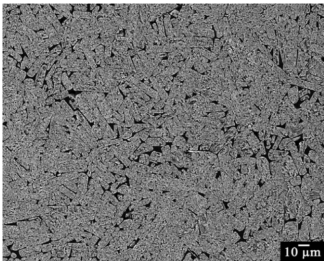
FIGURE 1 Microstructure of the sintered Ti_2AlC pellet
