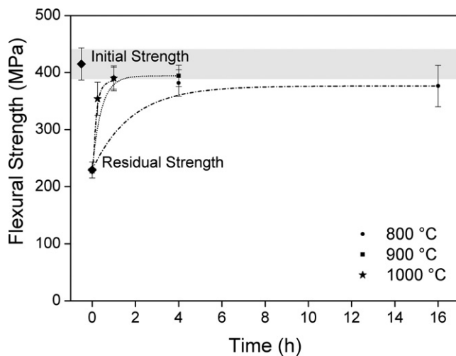
FIGURE 9 Flexural strength of studied materials attained by 4-point bending
