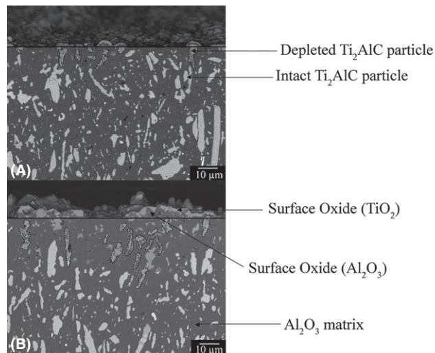
FIGURE 12 SEM cross-sectional view of the composite at 1000°C in air for (A) 64 and (B) 256 h showing the depletion of Ti and Al from the \text{Ti}_2\text{AlC} particles close to the sample surface
