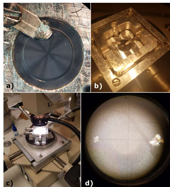
Fig. A.1. Illustration of the alignment method. a) Three small dots engraved on the top right side of the lens as the reference mark. b) In-house made alignment unit to position the HEB chip using two micrometer manipulators, where the HEB chip is pressed down on the back surface of the lens. c) The alignment unit mounted on the XY stage of a microscope. d) Example of a mark reference to register the chip orientation.
