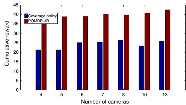
Fig. 12 Performance of POMDP-IR and the coverage policy on the shopping mall dataset (Color figure online)
