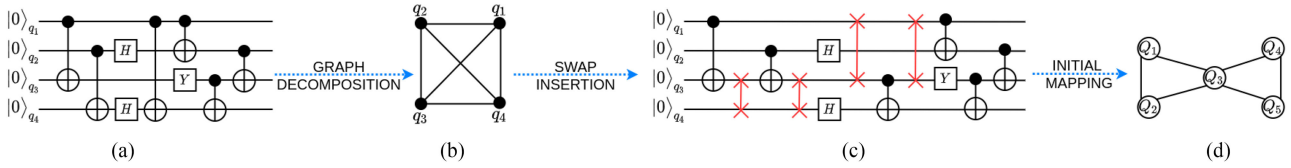
FIGURE 2. (a) Example quantum circuit. As shown in (b), this circuit is decomposed into a graph-theoretic version of the algorithm [also known as an interaction graph (IG) ] which illustrates the interaction via two-qubit gates of qubits in the original algorithm; edges represent two-qubit gates, while vertices represent qubits which are acted upon. Weights are added to vertices and edges in order to account for more gate invocations. In (c) the geometric connectivity of the IG is analyzed and SWAP gates are added for any interaction-graph edges which cannot be exactly assigned to the QPU coupling graph (CG); for example, if we define an assignment \{q_1 \mapsto Q_1, q_2 \mapsto Q_2, q_3 \mapsto Q_3\} , then the interaction-graph edge between q_1 and q_4 cannot be explicitly assigned, since Q_1 and Q_4 do not share an edge connection in the QPU CG shown in (d). The modified quantum circuit is then assigned to the QPU in (d); in this way, the appropriate vertices, in accordance with some metric to be defined, are assigned to the graph-theoretic object representing the quantum device (referred to as the CG of the QPU). In many types of qubit-mapping algorithms, qubits can then be arranged and mapped temporally , as well as spatially during the routing process [48], [49], [52]; for this reason, the final arrow between (c) and (d) carries the designation initial assignment .
