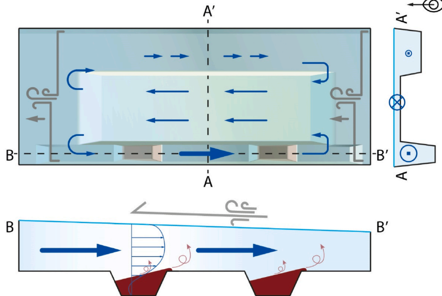
Fig. 8. Conceptual figure with topview (top left), lateral cross-section AA' (top right) and longitudinal cross-section BB' (bottom). Wind in longitudinal direction drives a horizontal circulation with downwind currents over the shallow part in the middle and upwind currents over the deeper parts, in particular the deep channel on the south side. When salt is present in the system, these currents can induce upwind salt transport, as observed in this study. For this, salt needs to be mixed upward from the deepest parts of the channel. We hypothesize the mixing mostly occurs when salt water – due to tilting of the pycnocline – reaches less deep parts of the channel, where it is subsequently more easily entrained by the wind-induced circulation.
