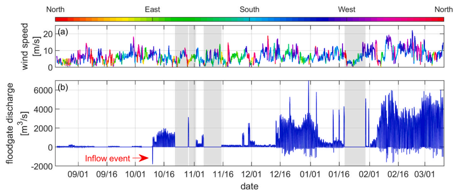
Fig. 2. Forcing conditions. Top) wind speed and direction (average of the preceding hour, directions following meteorological convention); Bottom) Estimated discharge through the floodgates (positive is seaward). The gray shades indicate multi-day periods of closed gates after the seawater inflow event on October 9, 2019. (For interpretation of the references to color in this figure legend, the reader is referred to the Web version of this article.)
