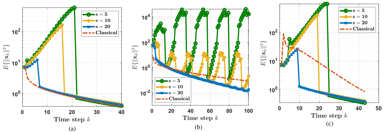
Fig. 2. Comparison of stabilization of an LDS with n = m = 50 , p = 12 , and n_1 = n_2 = 25 using sparse inputs with sparsity levels s = 5, 10 , and 20 . The behavior of conventional stabilization using nonsparse inputs is also shown. (a) Stabilization of noiseless LDS. (b) Mean-square stabilization of noisy LDS. (c) Stabilization of noiseless LDS through output feedback.
