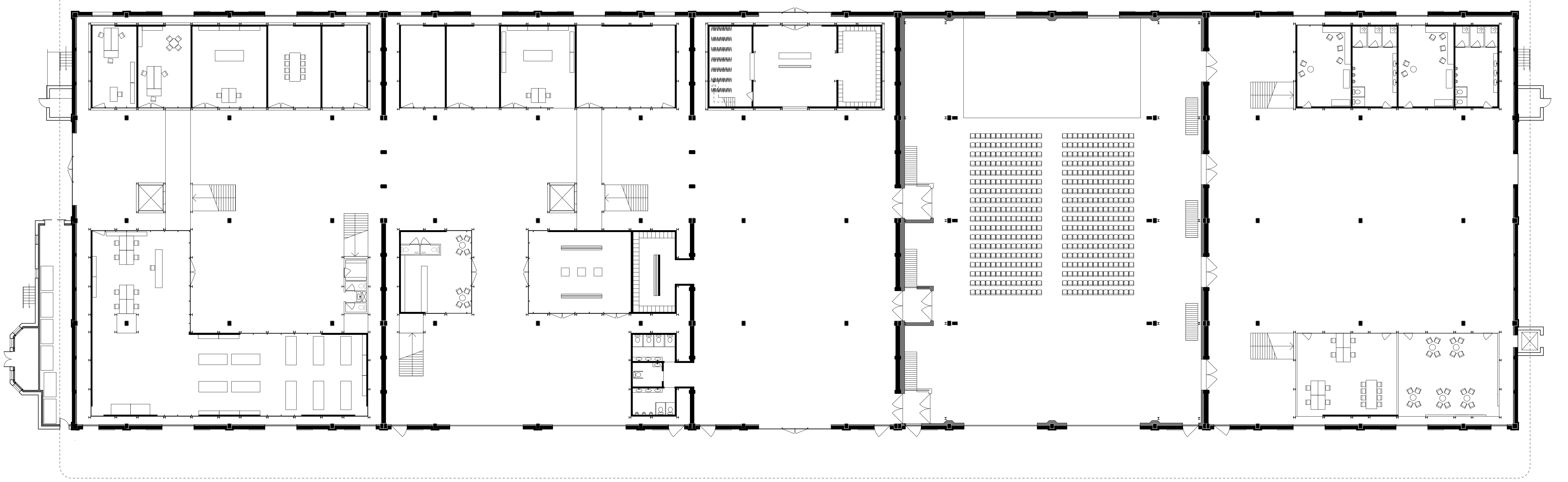
Ground floor plan 1:200
