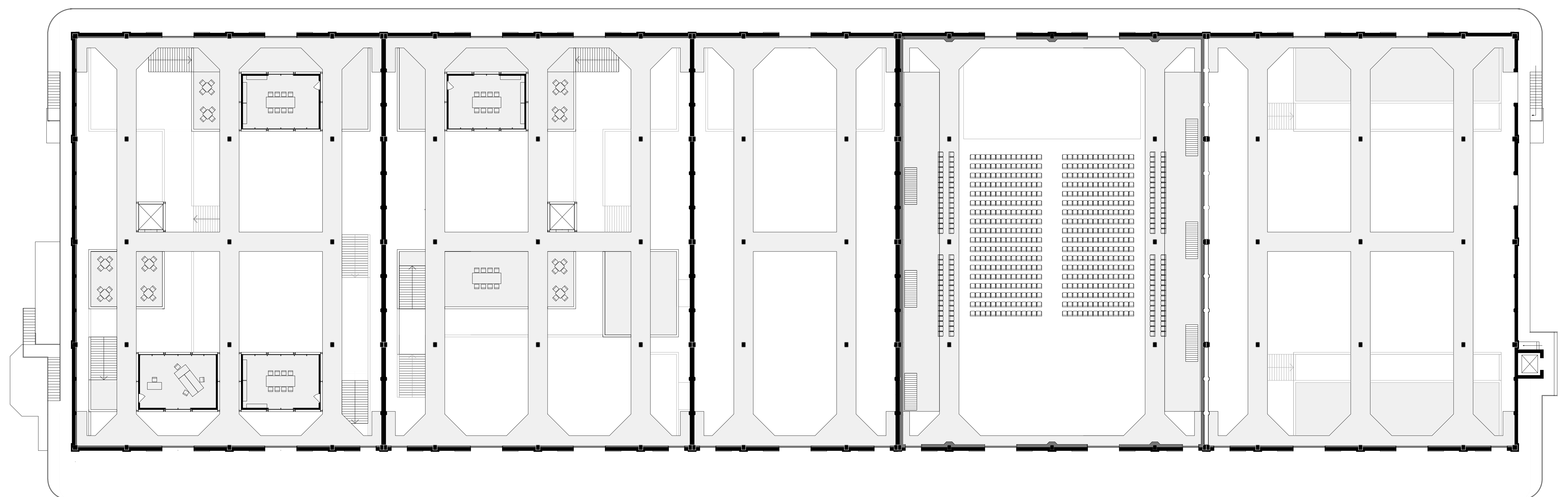
Second floor plan 1:200
