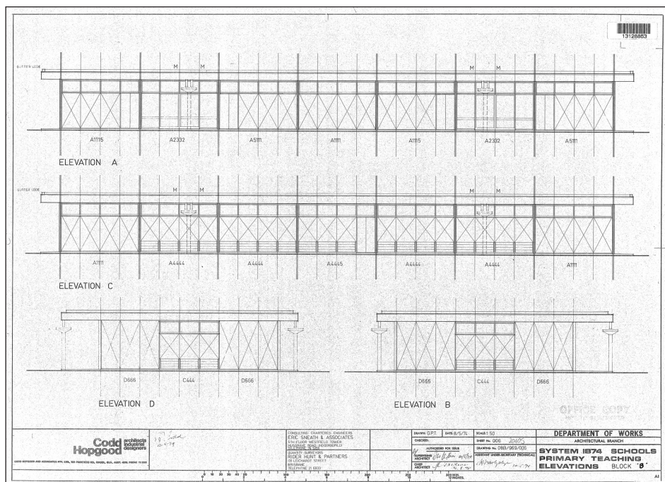
Figure 2: System IB74 schools, Elevations, designed by Codd Hopgood and Associates, 1974. Queensland State Archives (Brisbane, Australia), series 1173, box number 802, item ID 595380.
