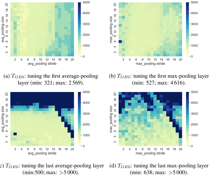
Figure 3.28: T_{GE0} for the standardized dataset for the HW leakage model on ASCAD.F.
