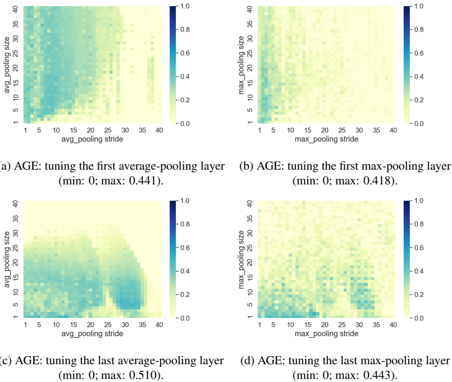
Figure 3.34: AGE for the HW leakage model on ASCAD_R.
