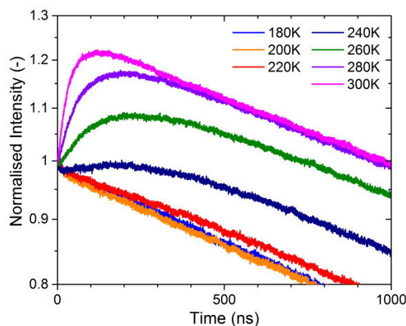
Figure 12: The decay spectra of emission A in NaBr:Tm 2+ plotted at a short time scale between 180 and 300K. The decay curves were acquired using pulsed laser excitation at 420nm and clearly exhibit a rise time phenomena for temperatures above 200K.
