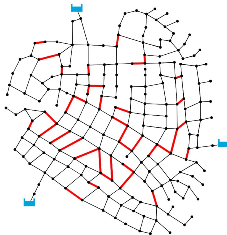
Figure 3. Conceptual cuts obtained for the three-reservoir network (TRN).
