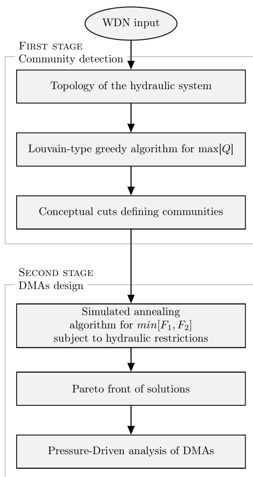
Figure 2. Conceptual flowchart of the procedure.
