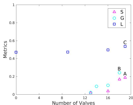
Figure 5. Pareto front of solutions for the three-reservoir network (TRN) obtained with the three studied performance indices (PIs). Legend: S: Standard deviation, G: Gini coefficient, L: Loss of resilience.
