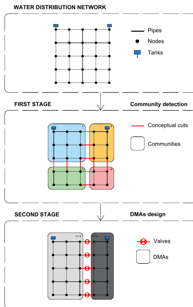
Figure 1. Schematic process of district metering areas (DMAs) design for a simple network.
