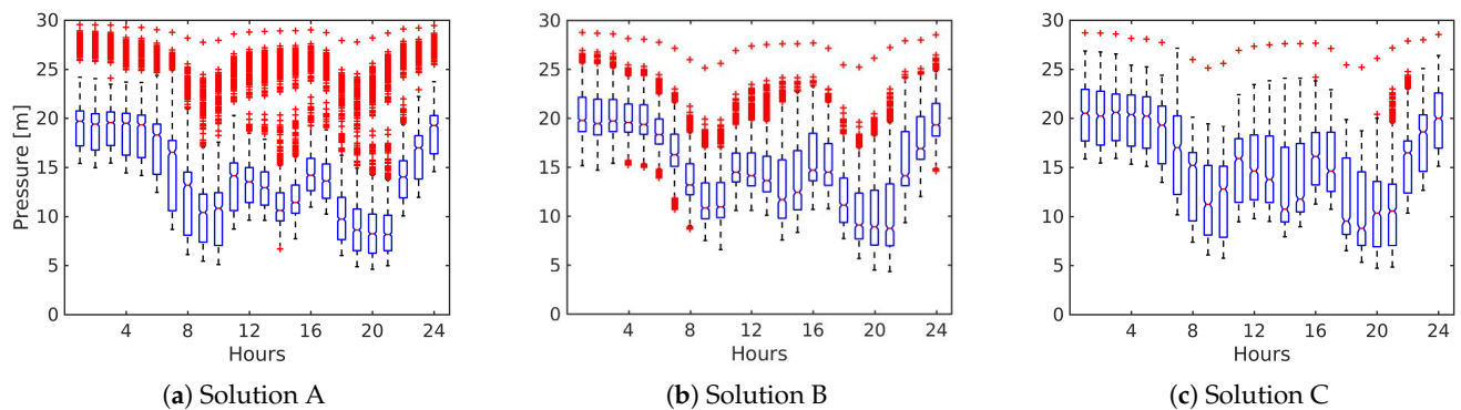
Figure 12. Temporal variation of pressure for solution A, B and C for MLN network. Each time step represents a box plot for the pressure of all nodes of the network.
