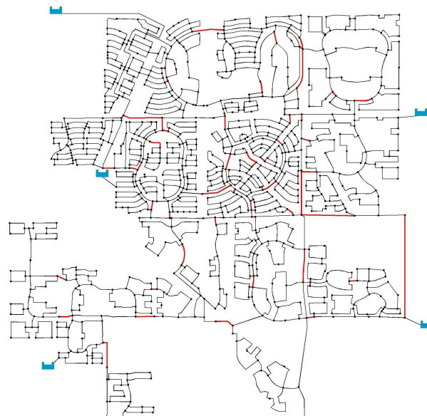
Figure 4. Conceptual cuts obtained for the modified large network (MLN).
