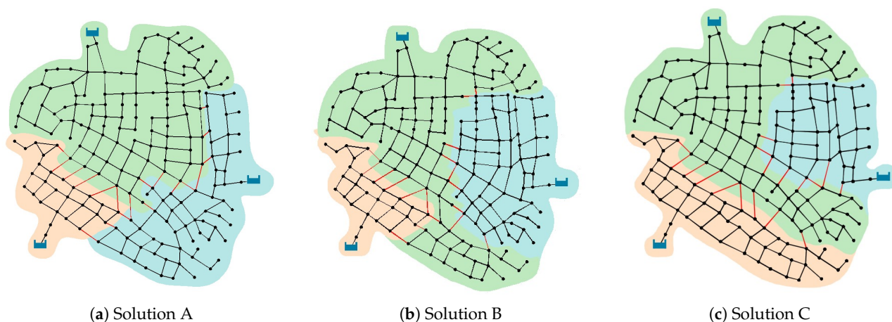
Figure 6. DMAs obtained after the second stage for each PI. (a) Standard deviation, (b) Gini coefficient and (c) Loss of resilience. Solutions correspond to those indicated in Figure 5 and to the gray color rows in Tables.
