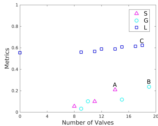
Figure 9. Pareto front of solutions for MLN network obtained with the three studied PIs. Legend: S: Standard deviation, G: Gini coefficient, L: Loss of resilience.
