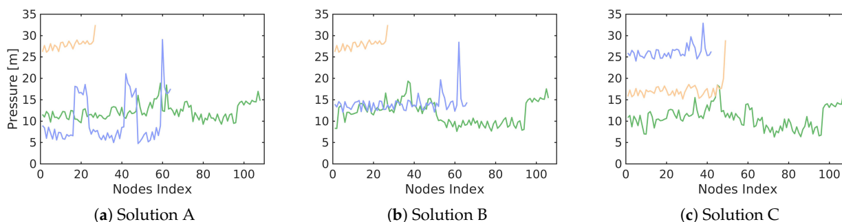
Figure 8. Nodal pressures for the solutions A, B and C for TRN network. Colors code corresponding to DMAs of Figures 6 and 7.
