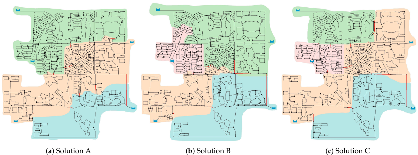
Figure 10. DMAs obtained for MLN network. Solutions A, B and C are those indicated in Figure 9 for (a) Standard deviation, (b) Gini coefficient and (c) Loss of resilience.
